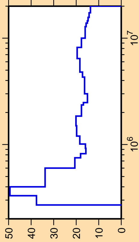
\Delta\sigma/\sigma vs. E for ^{249}\text{Bk}(n,n_{10})
