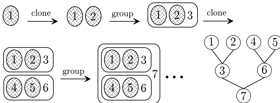
Figure 6.11: Schematic representation of the construction of an array of cells by progressively cloning and grouping modules obtained from a primary cell module. The labels of the modules are the internal labels assigned by PENGEOM . Notice the evolution of the modular tree at each step.
