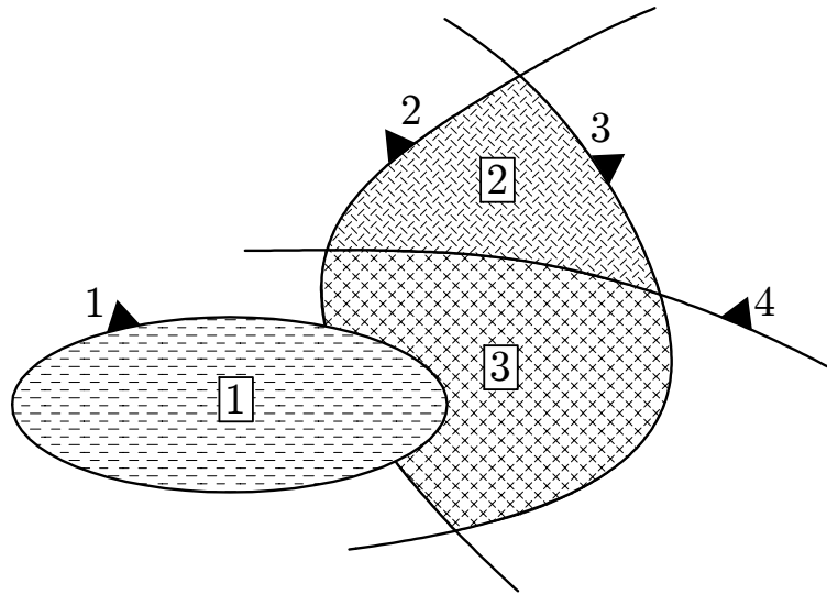
Figure 6.3: Schematic representation of a simple geometry. The solid triangles indicate the outside of the surfaces (side pointer = +1); numbers in squares indicate bodies.
