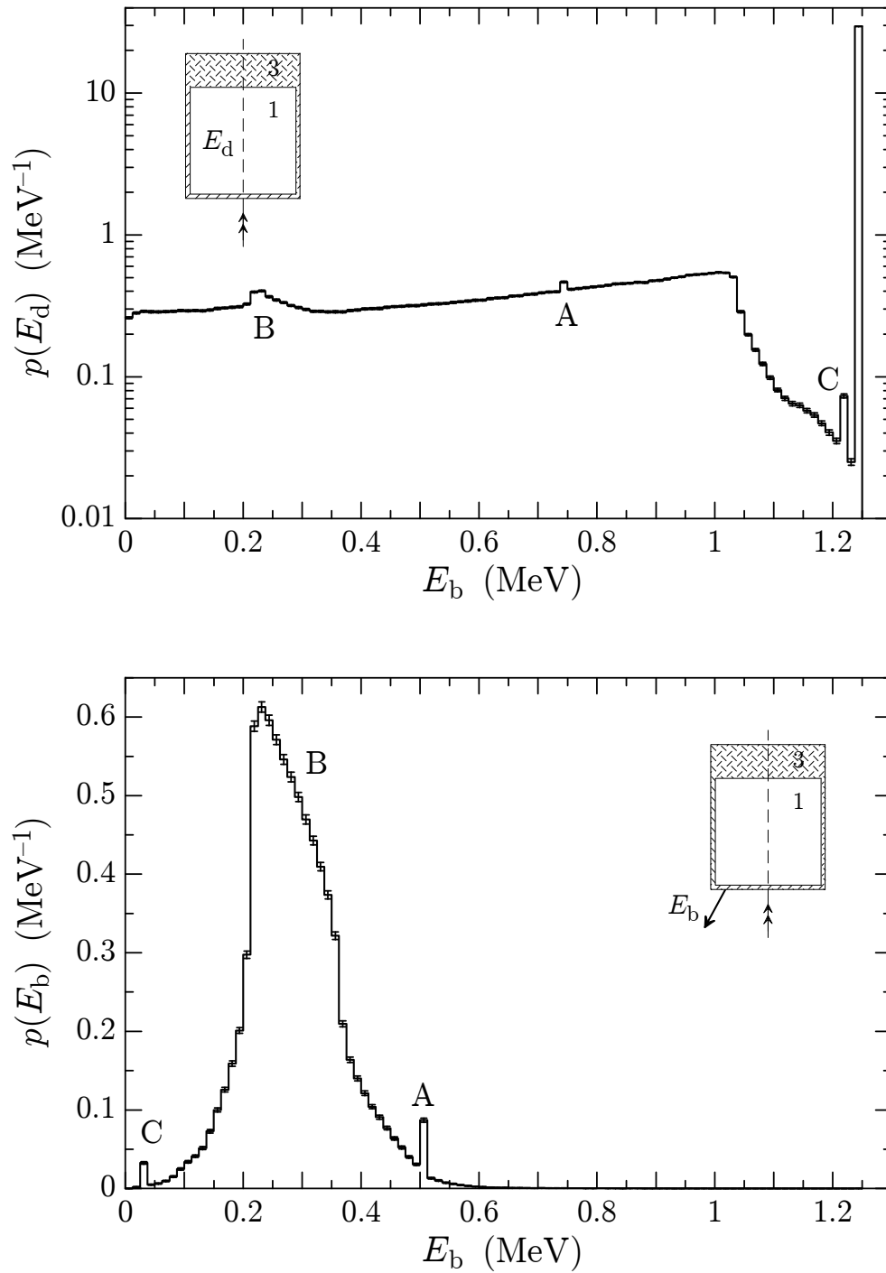
Figure 7.4: Partial results from pencyl for the NaI photon detector described in the text (input file cy1d.in ). Top: distribution of energy deposited in the NaI crystal ( MAT=1 ). Bottom: energy distribution of backscattered (downbound) photons.
