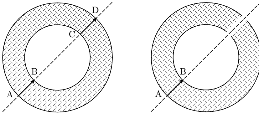
Figure 6.9: Tracking error caused by defining an enclosure that is concave. The example corresponds to a simple geometry consisting of a hollow cylinder in vacuum. The left diagram shows the correct tracking of a particle that crosses the material structure without interacting. When the hollow cylinder is defined as a body, the particle crosses the first wall (A–B), enters the hollow, moves freely to point C, and then crosses the second wall (C–D). If the hollow cylinder is defined as a module, PENGINE identifies it with the enclosure and the program malfunctions: the particle crosses the first wall (A–B), enters the hollow at B and, because it is in the vacuum, flies freely to infinity, failing to “see” the second wall.
