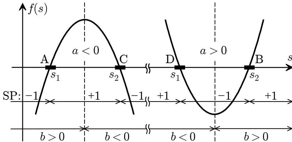
Figure 6.5: The intersections of a ray \mathbf{r}_0 + s\hat{\mathbf{d}} with a fuzzy quadric surface, described in terms of the variation of the master function, f(s) = as^2 + bs + c , Eq. (6.21). The path length s increases to the right. The roots s_1 and s_2 of the equation f(s) = 0 are the distances at which the ray intersects the surface, sorted in increasing order ( s_1 < s_2 ). The solid blocks (labelled A, B, C and D) indicate ray segments about the intersections with the surface where |f(s)| < \epsilon . When the initial point \mathbf{r}_0 lies in one of these segments, the sign of f(s) , that is, the SP of the surface at \mathbf{r}_0 , may be ambiguous because of floating-point round-off errors. The ambiguity can be resolved by considering the sign of b [ i.e. , of the derivative of f(s) at s = 0 ], and the existence of a second crossing ahead can be recognized from the sign of a , as described in the text.
