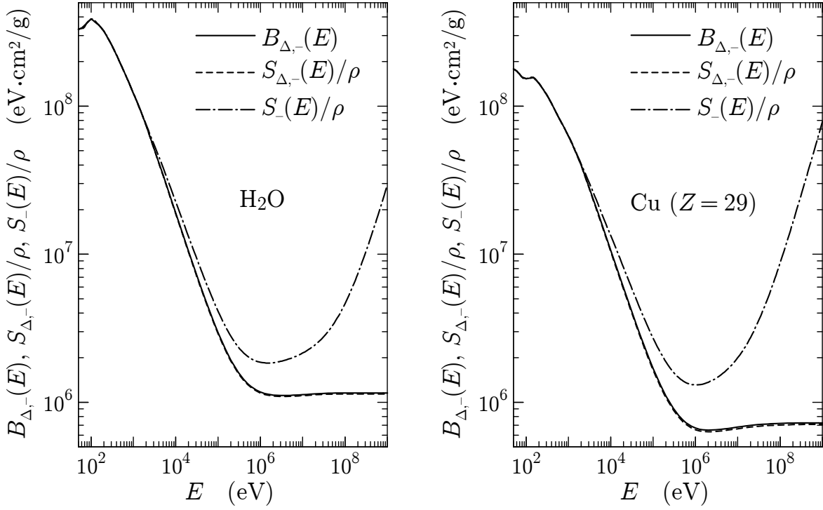
Figure 5.2: Mass energy absorption, B_{\Delta,-}(E) , restricted mass stopping power, S_{\Delta,-}(E)/\rho , and mass stopping power, S_-(E)/\rho , of electrons in water and copper, calculated with \Delta_- = \Delta_+ = 1 keV and \Delta_\gamma = 0 . For projectiles with energies less than about 10 keV, the MEA practically coincides with the restricted mass stopping power.
