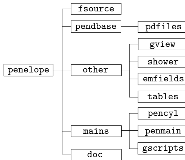
Figure 7.7: Directory tree of the PENELOPE code system.
