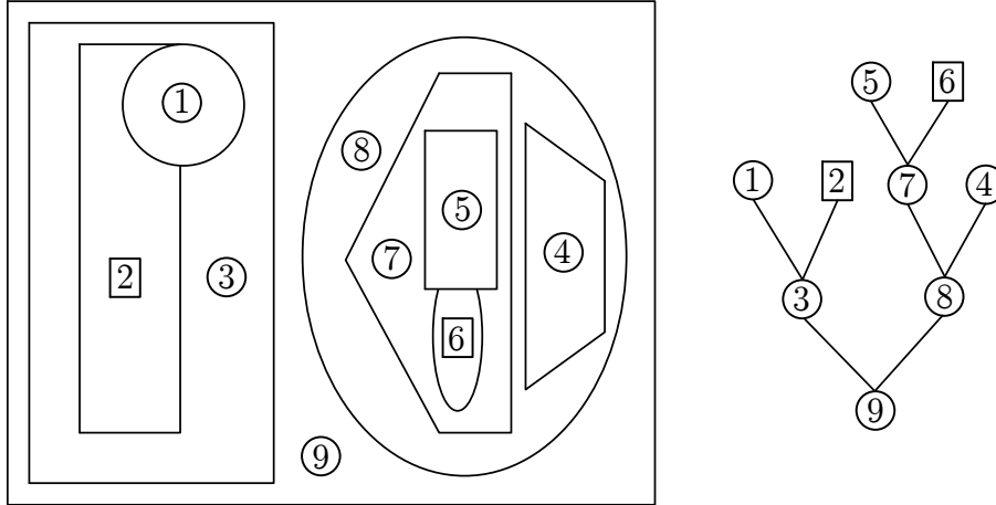
Figure 6.8: Planar cut of a geometry example, showing modules (number labels in circles) and bodies (number labels in squares), and the associated genealogical tree. Notice that a module can always be defined as a body limited by their submodules and daughter bodies, but this affects the structure of the genealogical tree and, therefore, the efficiency (speed) of the geometry operations.
