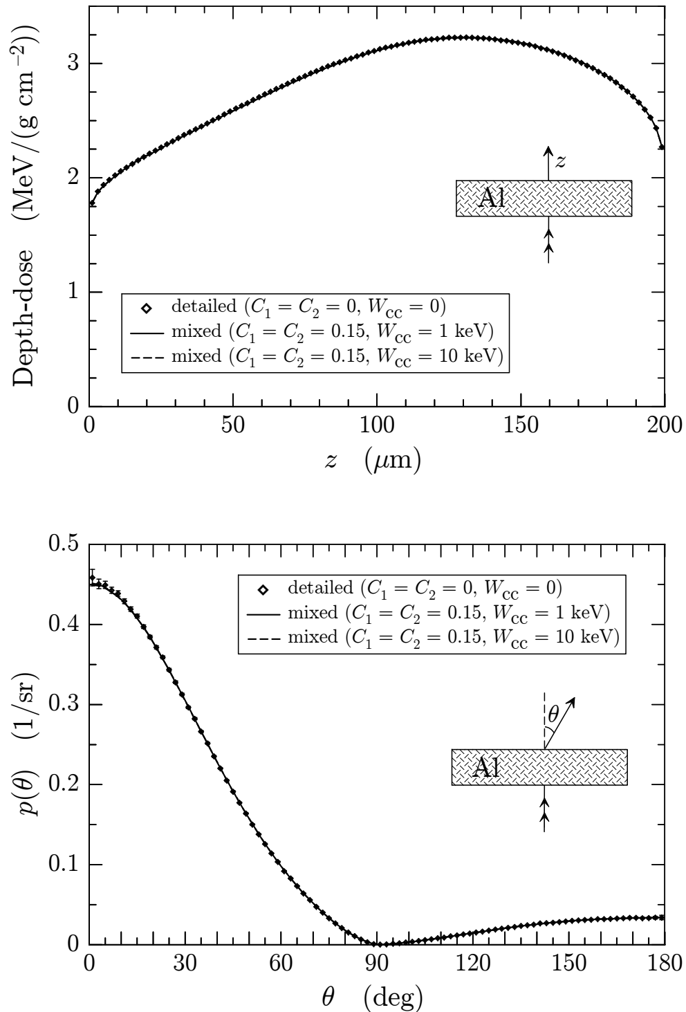
Figure 7.5: Results from pency1 for a 500 keV electron beam impinging normally on the surface of a 200- \mu\text{m} -thick aluminium slab (further details are given in the text). Top: depth-dose distribution within the slab. Bottom: angular distribution of emerging (transmitted and backscattered) electrons (primaries and secondaries).
