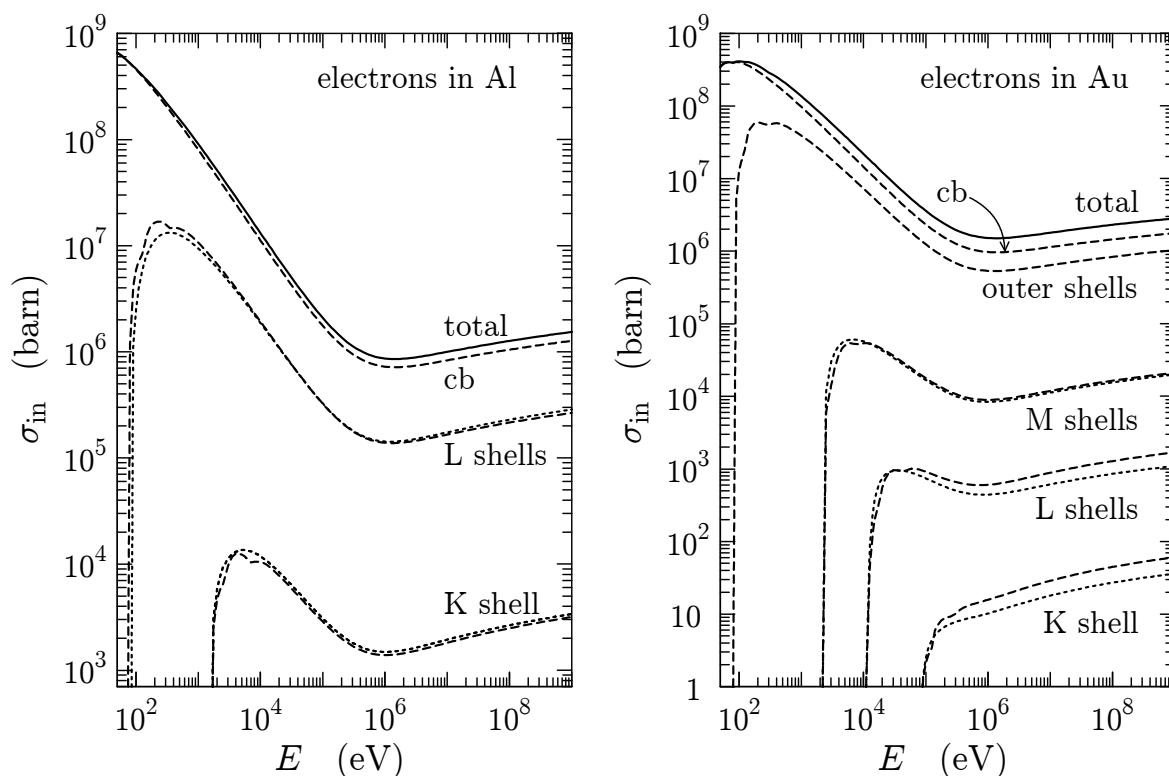
Figure 3.9: Total inelastic cross sections for electrons in aluminium and gold and contributions from the K shell, L and M shells, conduction band (cb) and outer shells, calculated from our model GOS ignoring density effect corrections ( i.e. , with \delta_F = 0 ). In the calculations we used the following values of the oscillator strength and the resonance energy for conduction-band excitations: f_{cb} = 3 and W_{cb} = 15.8 eV for aluminium, and f_{cb} = 11 and W_{cb} = 40 eV for Au. The dotted curves represent ionisation cross sections for the K shell and the L and M shells taken from the numerical database described in Section 3.2.6. Note: 1 barn= 10^{-24} cm 2 .
