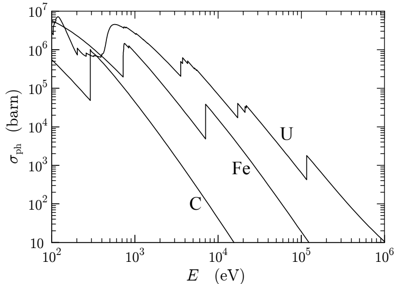
Figure 2.4: Atomic photoelectric cross sections for carbon, iron and uranium as functions of the photon energy E .
