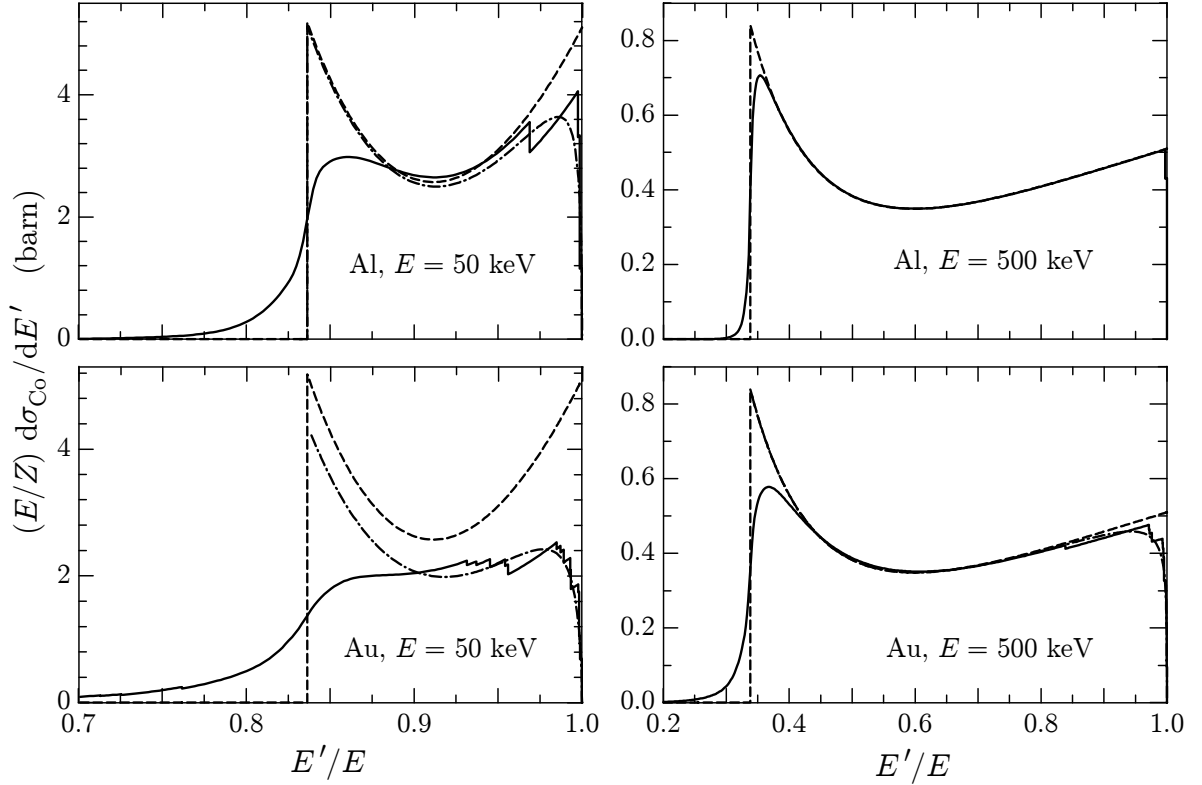
Figure 2.9: Energy DCSs for Compton scattering of 50 and 500 keV photons by aluminium and gold atoms. The continuous curves represent the DCS (2.49), computed using the analytical Compton profiles (2.54). The dashed curves are obtained from the Klein-Nishina formula (2.50), i.e. , assuming that the atomic electrons are free and at rest. Dot-dashed curves represent results from the Waller-Hartree theory, Eq. (2.51). (Adapted from Brusa et al. , 1996.)
