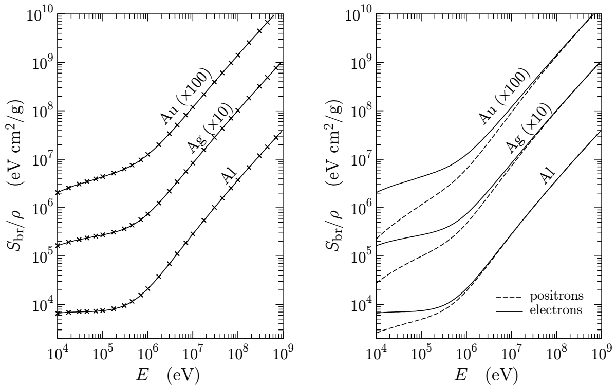
Figure 3.14: Radiative stopping power S_{\text{br}}/\rho for electrons and positrons in aluminium, silver ( \times 10 ) and gold ( \times 100 ) as a function of the kinetic energy. Solid and dashed curves are results from the present model. Crosses are data from the ICRU Report 37 (1984) (given also in Berger and Seltzer, 1982).
