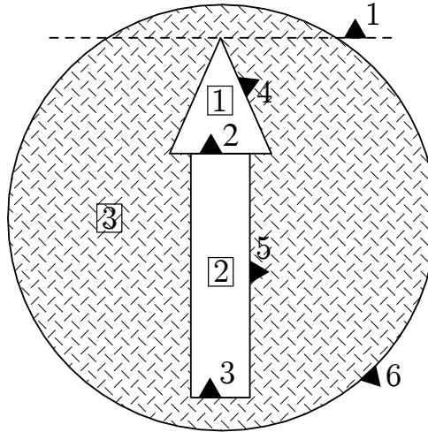
Figure 6.7: Example of simple quadric geometry; an arrow within a sphere (the corresponding definition file is given in Section 6.7). The solid triangles indicate the outside of the surfaces (side pointer SP = +1 ). Numbers in squares indicate bodies.
