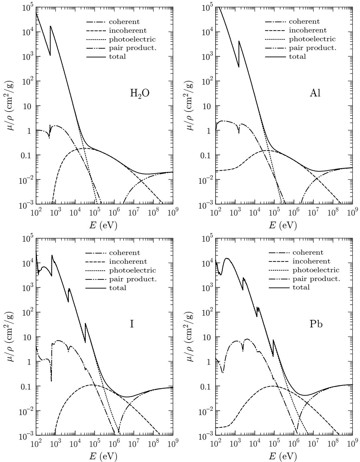
Figure 2.12: Partial and total mass attenuation coefficients of water, aluminium, iodine and lead as functions of the photon energy. Notice the different low- E behaviour of \mu_{\text{Co}}/\rho for insulators (water and iodine) and conductors (aluminium and lead).
