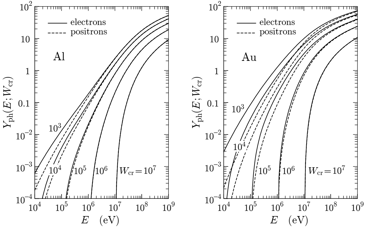
Figure 3.18: Photon number yields of electrons and positrons in aluminium and gold, for the indicated values of the cutoff energy W_{\text{cr}} , as functions of the kinetic energy E .
