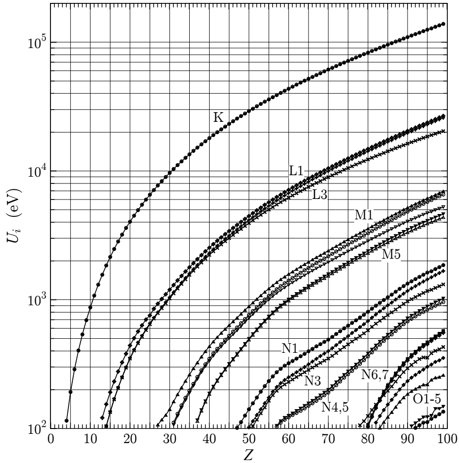
Figure 2.3: Shell ionisation energies of neutral atoms, U_i , in eV. Symbols represent values given by Carlson (1975), joined by straight segments for visual aid.
