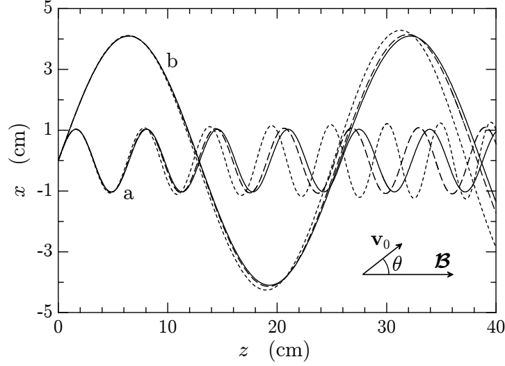
Figure D.3: Trajectories of electrons and positrons in a uniform magnetic field of 0.2 tesla. Continuous curves are exact trajectories calculated from Eq. (D.30). The short-dashed lines are obtained by using the numerical tracking method described in the text with \delta_v = 0.02 . Long-dashed curves are the results from the tracking algorithm with \delta_v = 0.005 . a: electrons, E_0 = 0.5 MeV, \theta = 45 deg. b: positrons, E_0 = 3 MeV, \theta = 45 deg.
