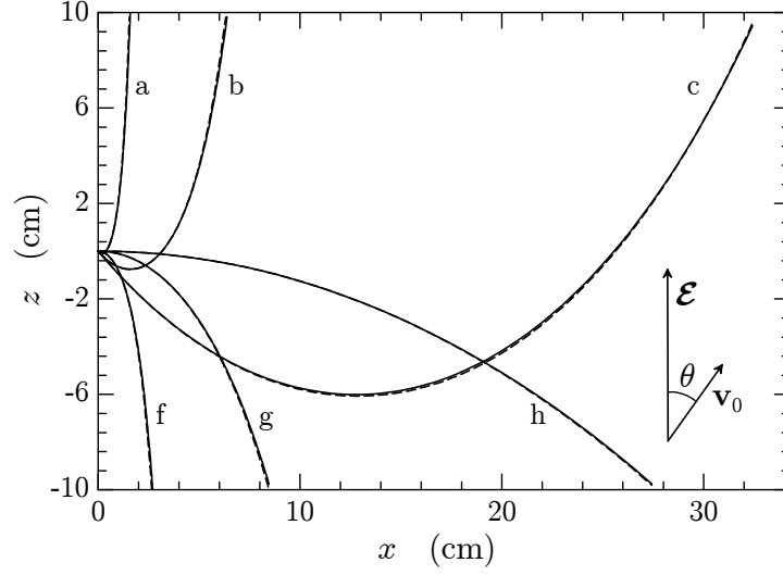
Figure D.1: Trajectories of electrons and positrons in a uniform electric field of 511 kV/cm. Continuous curves represent exact trajectories obtained from Eq. (D.21). The dashed lines are obtained by using the first-order numerical tracking method described by Eqs. (D.14)–(D.20) with \delta\boldsymbol{\mathcal{E}} = \delta E = \delta v = 0.02 . The displayed trajectories correspond to the following cases. a: positrons, E_0 = 0.1 MeV, \theta = 135 deg. b: positrons, E_0 = 1 MeV, \theta = 135 deg. c: positrons, E_0 = 10 MeV, \theta = 135 deg. f: electrons, E_0 = 0.2 MeV, \theta = 90 deg. g: electrons, E_0 = 2 MeV, \theta = 90 deg. h: electrons, E_0 = 20 MeV, \theta = 90 deg.
