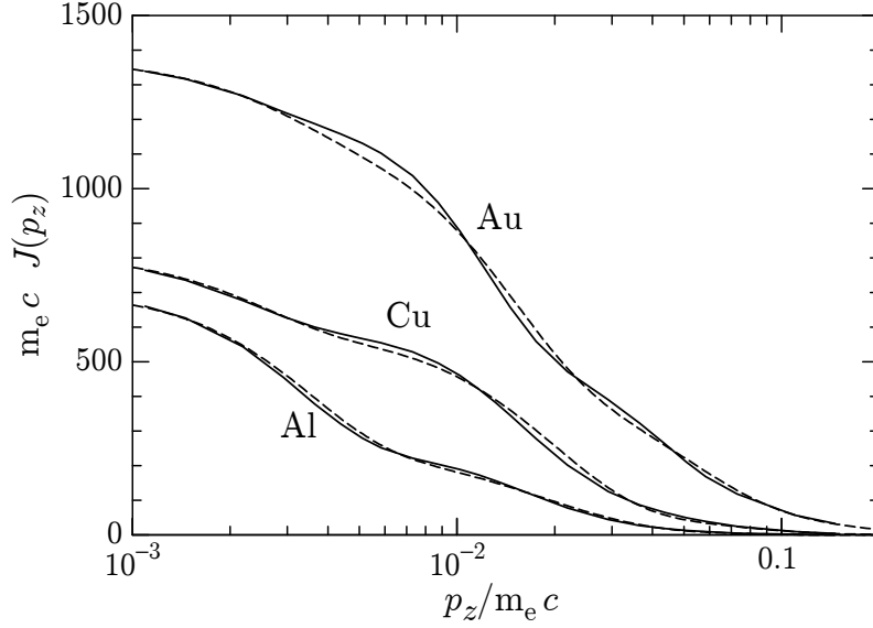
Figure 2.7: Atomic Compton profiles ( p_z > 0 ) for aluminium, copper and gold. The continuous curves are numerical Hartree-Fock profiles tabulated by Biggs et al. (1975). The dashed curves represent the analytical profiles defined by Eq. (2.54). (Adapted from Brusa et al. , 1996.)
