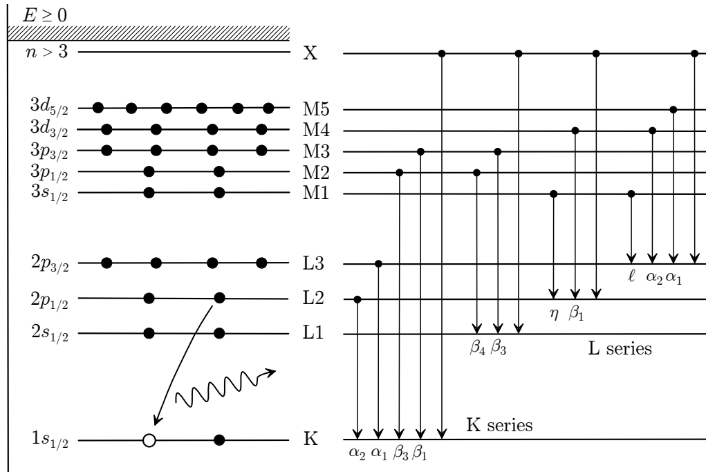
Figure 2.2: Various notations for inner atomic electron shells (left) and allowed radiative transitions (right) to these shells. Transitions that are different from the ones indicated in the diagram ( e.g. , K-M4) are also possible, but their transition probabilities are extremely small.
