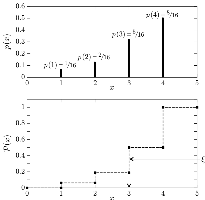
Figure 1.2: Random sampling from a discrete PDF using the inverse-transform method. The random variable can take the values i = 1, 2, 3 and 4 with relative probabilities 1, 2, 5 and 8 , respectively.
