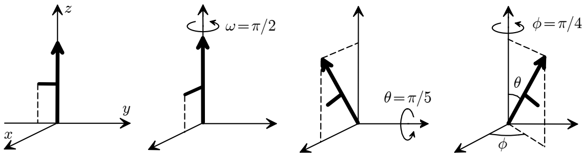
Figure 6.1: Rotation of an asymmetric object, an arrow with a protuberance, as defined by the Euler angles \omega , \theta , and \phi . The orientation of the axes is the same in all the diagrams.
