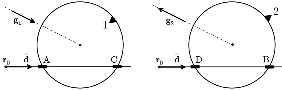
Figure 6.4: Intersections of rays \mathbf{r}_0 + s\hat{\mathbf{d}} with two quadric surfaces, which for simplicity are represented as spheres. The solid triangles indicate the outside of the surfaces ( SP = +1 ). The two surfaces differ only in their orientation ( i.e. , their defining functions differ by a global negative factor) and, consequently, their gradient vectors \mathbf{g}_i = \nabla F_i(\mathbf{r}) are in opposite directions. The SP of a surface at \mathbf{r}_0 may be ambiguous when |F(\mathbf{r}_0)| < \epsilon , i.e. , when the point lies close to the surface. The ray segments where this occurs have been indicated by solid blocks, not to scale.
