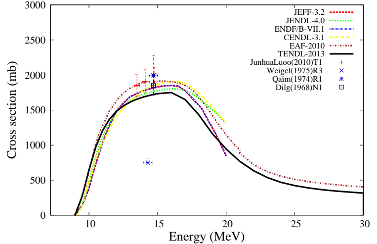
^{154}\text{Gd}(n,2n)^{153}\text{Gd}
