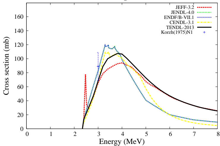
^{48}\text{Ti}(n,n_2')^{48}\text{Ti}
