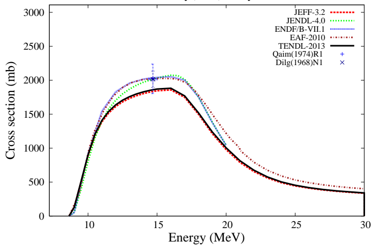
^{160}\text{Dy}(n,2n)^{159}\text{Dy}
