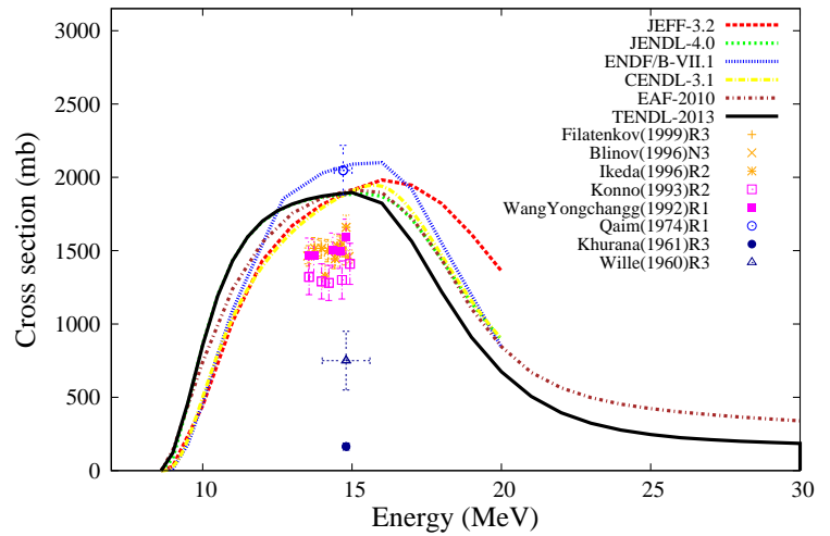
^{153}\text{Eu}(n,2n)^{152\text{m}}\text{Eu}
