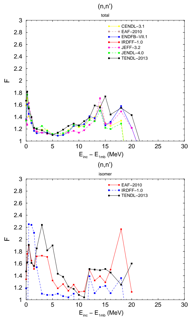
Figure 12: F values, averaged over all nuclides, for (n,n') reactions as a function of incident energy, for the various nuclear data libraries. E_{1mb} is an estimate for the threshold energy and is the incident energy where the cross section crosses the 1 mb value.
