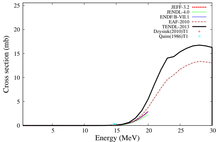
^{176}\text{Yb}(n,n\alpha)^{172}\text{Er}
