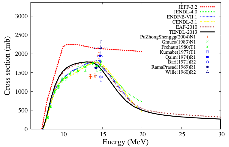
^{144}\text{Sm}(n,2n)^{143}\text{Sm}
