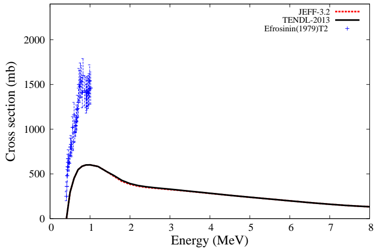
^{198}\text{Hg}(n,n_1)^{198}\text{Hg}
