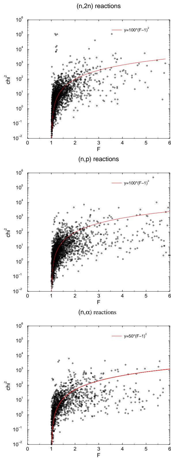
Figure 8: \chi^2 values as function of the F values for three reaction classes. The solid line is an eye-guide for the average behavior.
