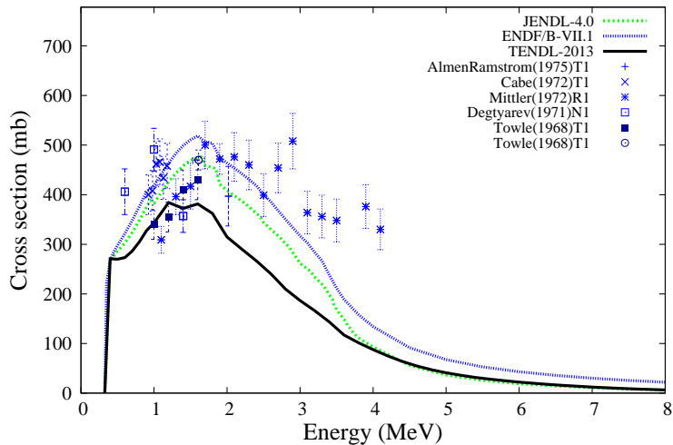
^{53}\text{Cr}(n,n_1)^{53}\text{Cr}
