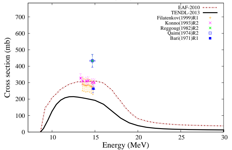
^{154}\text{Gd}(n,2n)^{153}\text{Gd}
