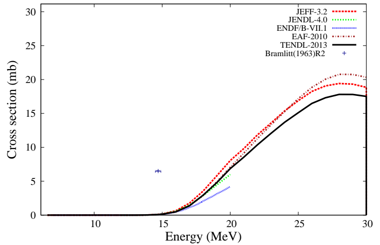
^{91}\text{Zr}(n,\text{na})^{87\text{m}}\text{Sr}
