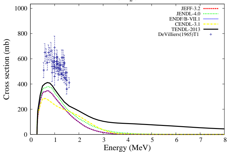
^{205}\text{Tl}(n,n_2')^{205}\text{Tl}
