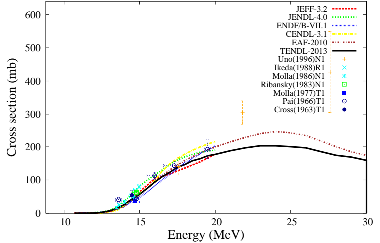
^{47}\text{Ti}(n,np)^{46m}\text{Sc}
