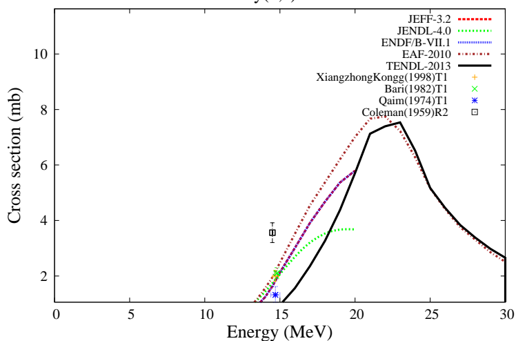
^{162}\text{Dy}(n,a)^{159}\text{Gd}
