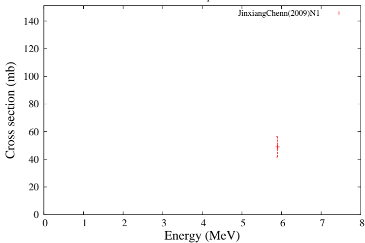
{}^9\text{Be}(n,n_1){}^9\text{Be}
