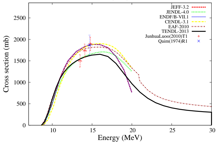
^{152}\text{Gd}(n,2n)^{151}\text{Gd}
