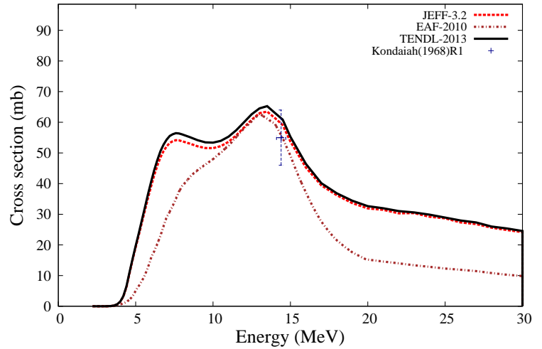
^{84}\text{Kr}(n,p)^{84g}\text{Br}
