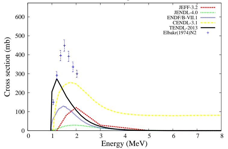
^{238}\text{U}(n,n_6')^{238}\text{U}
