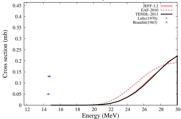
^{50}\text{Ti}(n,2p)^{49}\text{Ca}
