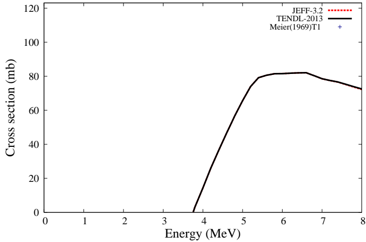
^{27}\text{Al}(n,n_2')^{27}\text{Al}
