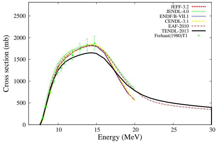
^{150}\text{Nd}(n,2n)^{149}\text{Nd}
