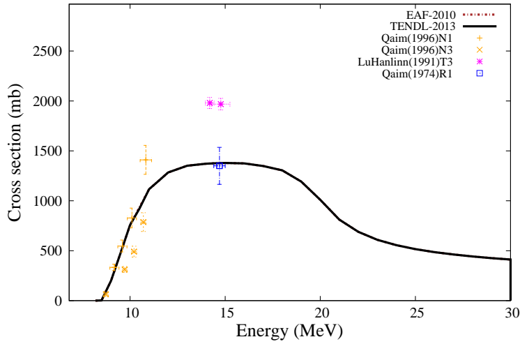
^{156}\text{Dy}(n,2n)^{155}\text{Dy}
