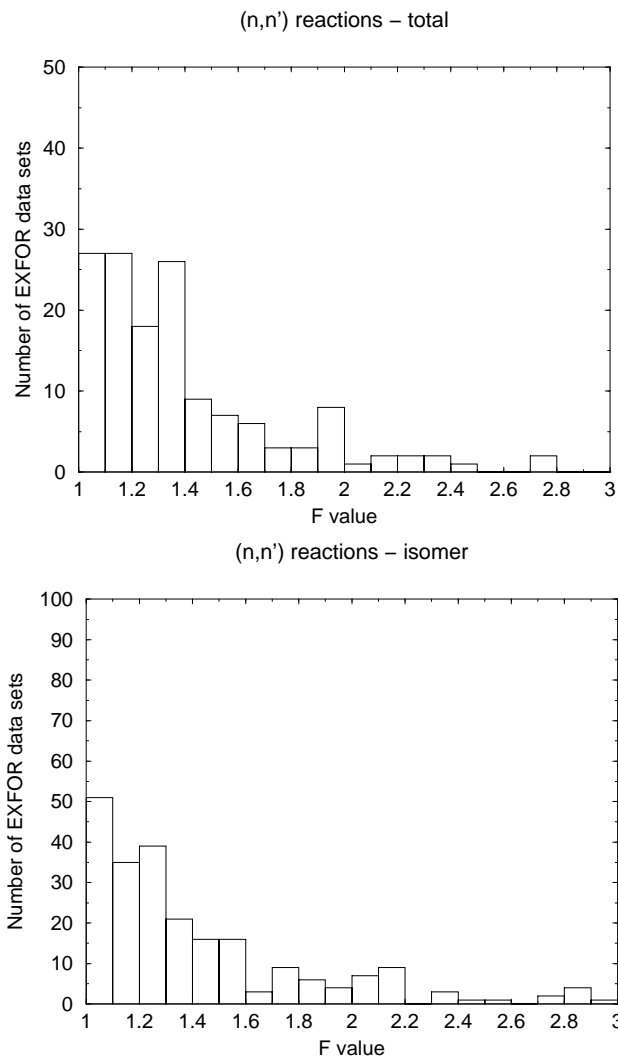
Figure 5: Distribution of F-values for the (n,n') reaction.
