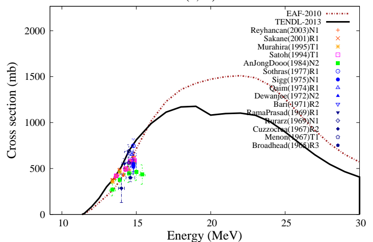
^{144}\text{Sm}(n,2n)^{143m}\text{Sm}
