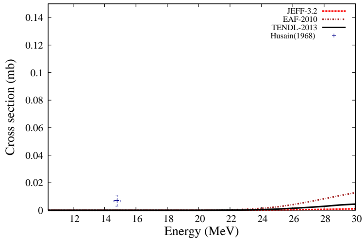
^{133}\text{Cs}(n,2p)^{132}\text{I}
