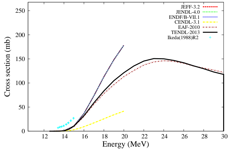
^{27}\text{Al}(n,np)^{26}\text{Mg}
