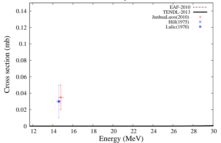
^{139}\text{La}(n,2p)^{138}\text{Cs}
