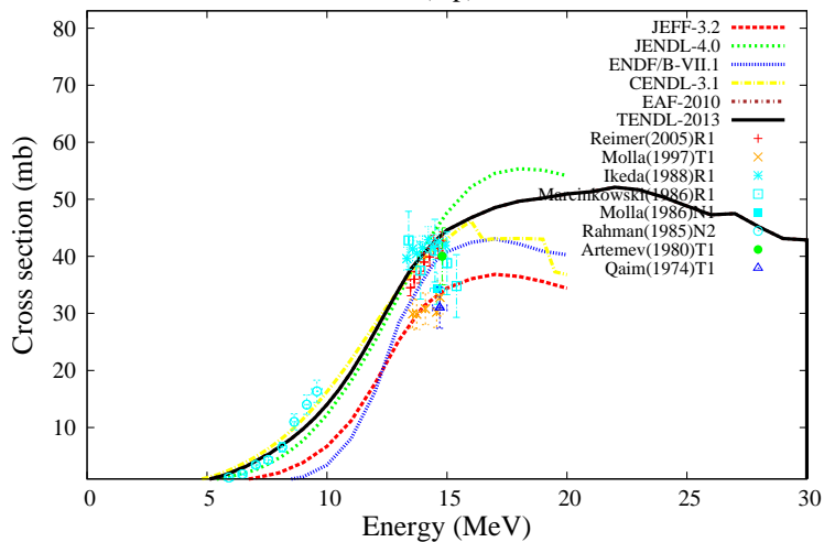
^{95}\text{Mo}(n,p)^{95m}\text{Nb}
