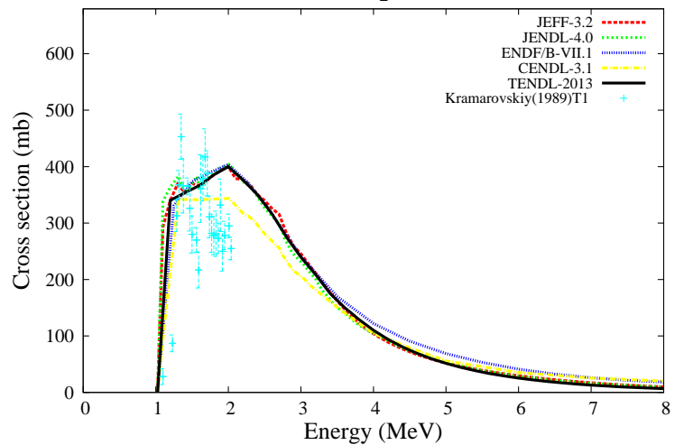
^{53}\text{Cr}(n,n_2')^{53}\text{Cr}
