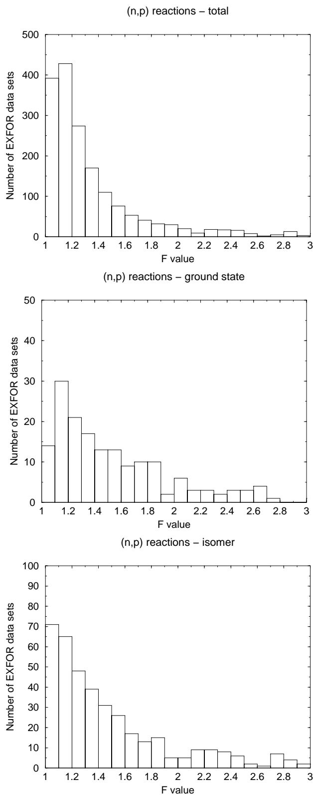
Figure 3: Distribution of F-values for the (n,p) reaction.
