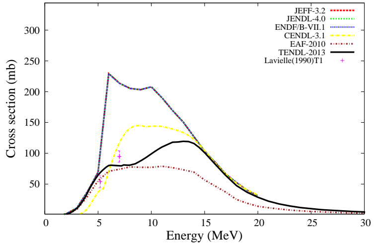
^{26}\text{Al}(n,a)^{23}\text{Na}
