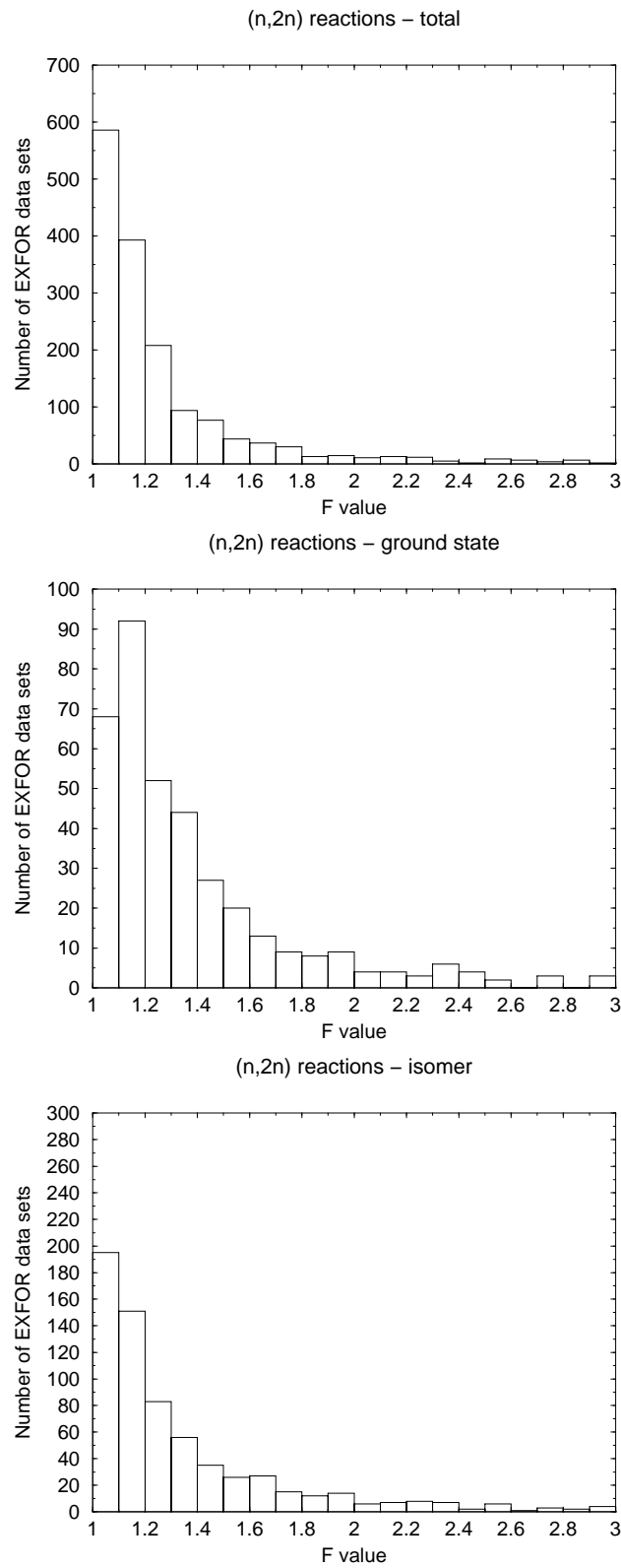
Figure 2: Distribution of F-values for the (n,2n) reaction.
