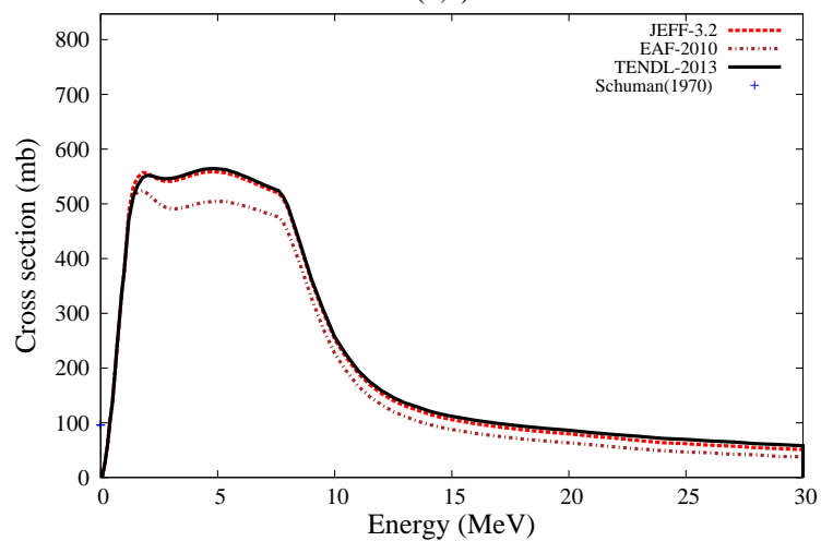
^{60}\text{Co}(n,n)^{60\text{m}}\text{Co}
