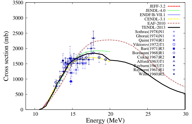
^{144}\text{Sm}(n,2n)^{143m}\text{Sm}
