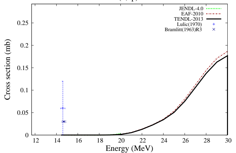
^{51}\text{V}(n,2p)^{50}\text{Sc}
