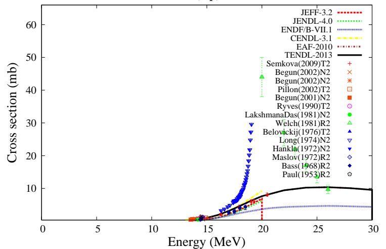
^{235}\text{U}(n,p)^{235}\text{Pa}
