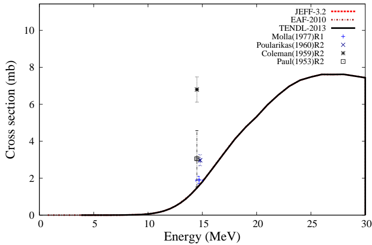
^{207}\text{Pb}(n,p)^{207}\text{Tl}
