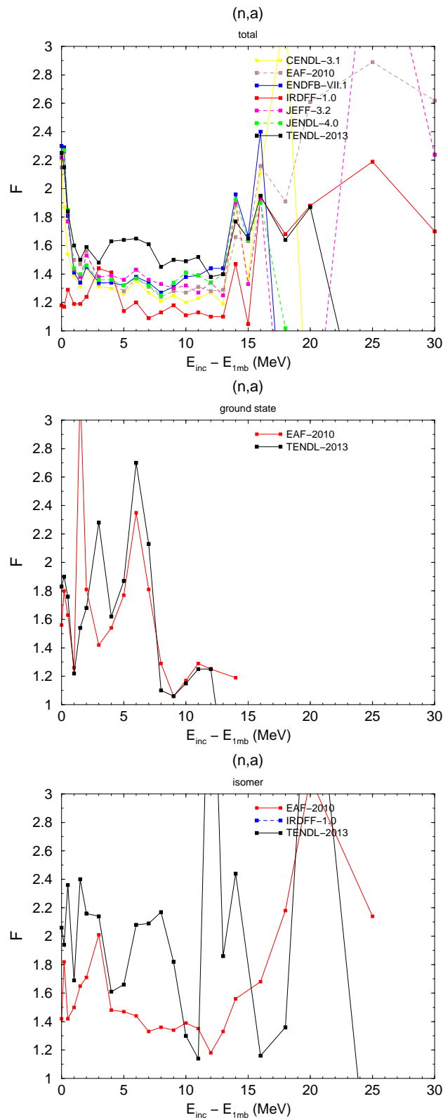
Figure 11: F values, averaged over all nuclides, for (n, \alpha ) reactions as a function of incident energy, for the various nuclear data libraries. E_{1mb} is an estimate for the threshold energy and is the incident energy where the cross section crosses the 1 mb value.
