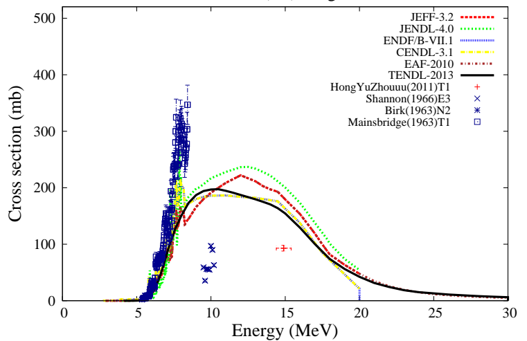
^{28}\text{Si}(n,a)^{25}\text{Mg}
