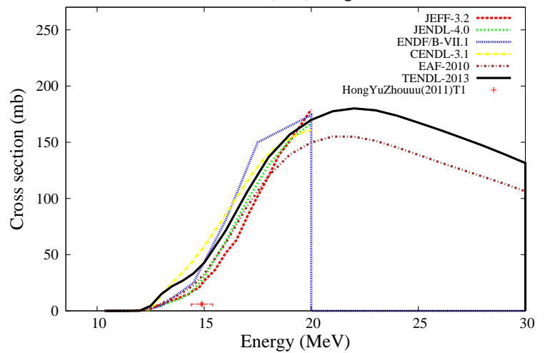
^{28}\text{Si}(n,\alpha)^{24}\text{Mg}
