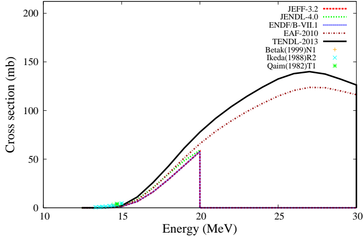
^{47}\text{Ti}(n,np)^{46g}\text{Sc}
