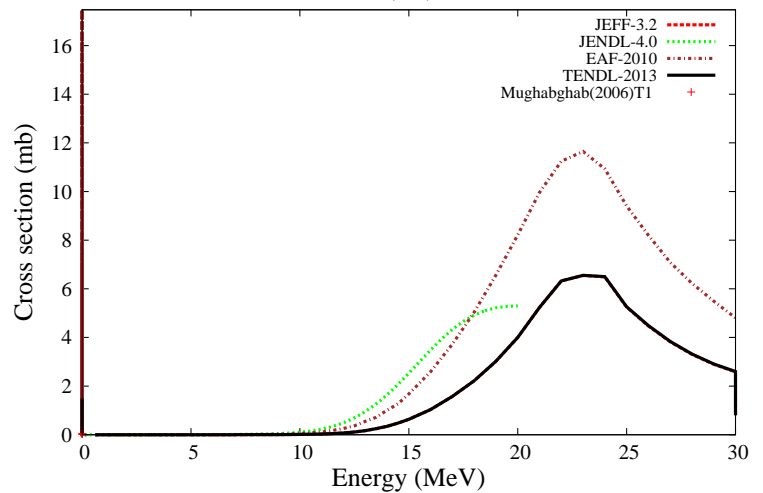
^{188}\text{Os}(n,a)^{185}\text{W}
