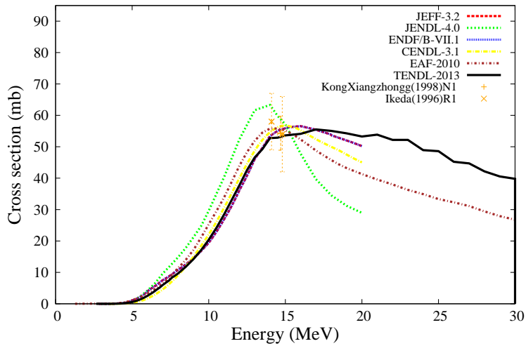
^{95}\text{Mo}(n,p)^{95}\text{Nb}
