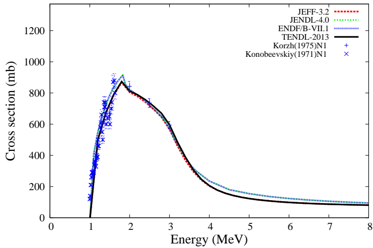
^{68}\text{Zn}(n,n_1')^{68}\text{Zn}
