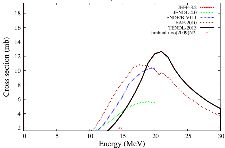
^{162}\text{Dy}(n,a)^{159}\text{Gd}
