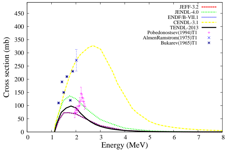
^{152}\text{Sm}(n,n_2')^{152}\text{Sm}
