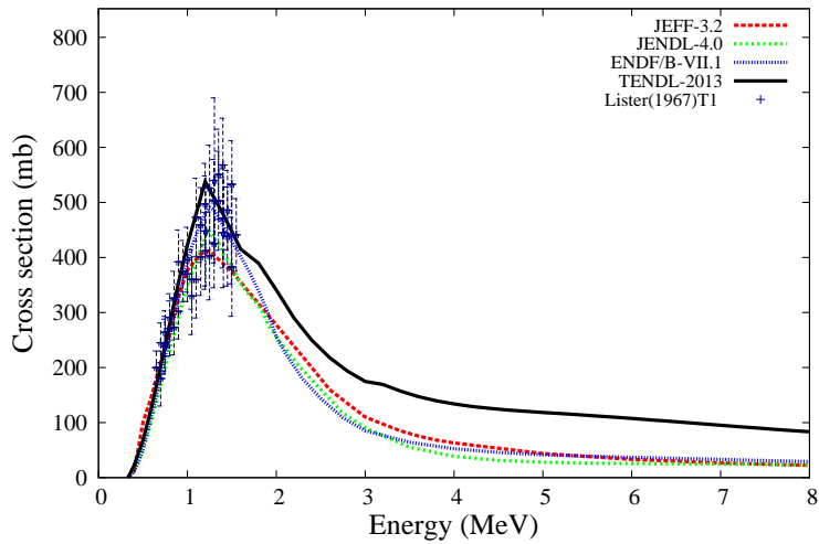
^{197}\text{Au}(n,n_2')^{197}\text{Au}
