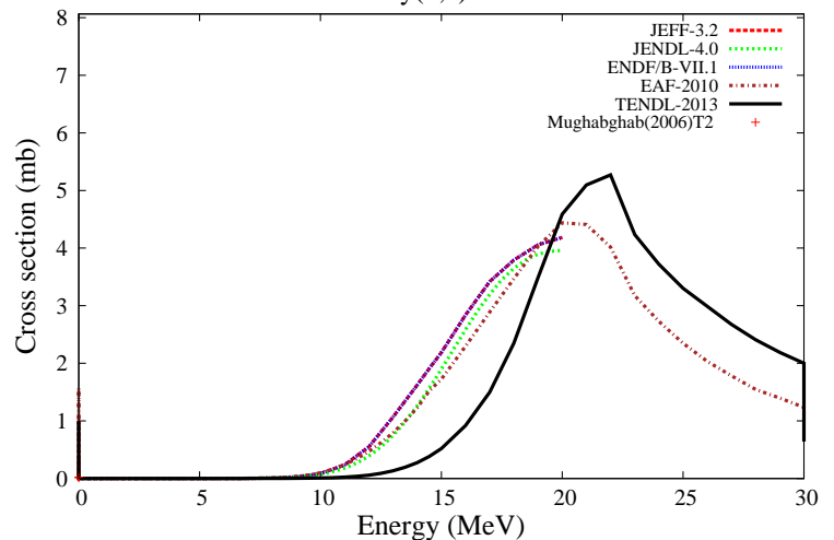
^{163}\text{Dy}(n,a)^{160}\text{Gd}
