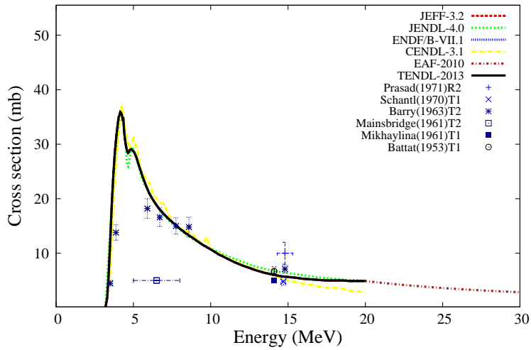
{}^9\text{Be}(n,p){}^9\text{Li}
