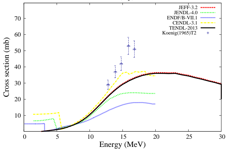
^{nat}\text{Rb}(n,p)\text{Kr}
