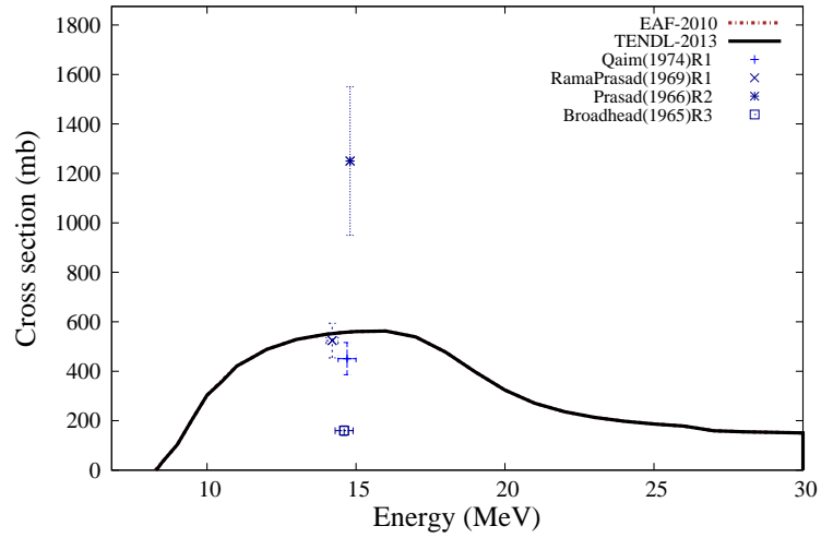
^{158}\text{Dy}(n,2n)^{157}\text{Dy}
