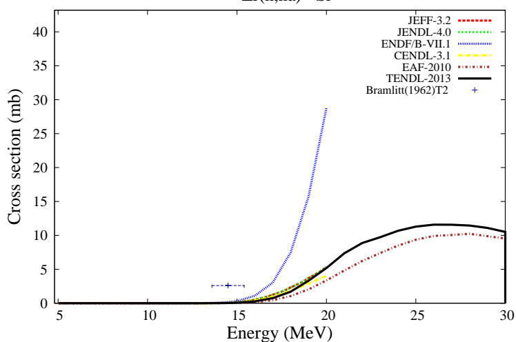
^{96}\text{Zr}(n,\text{na})^{92}\text{Sr}
