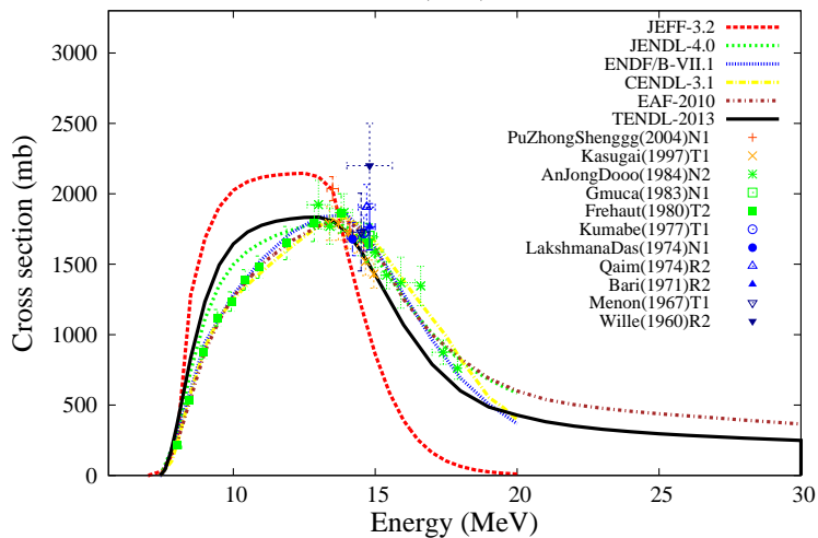
^{144}\text{Sm}(n,2n)^{143g}\text{Sm}
