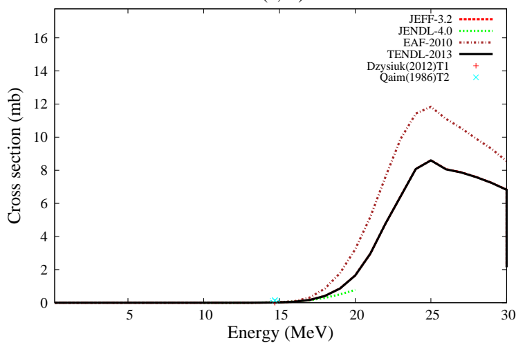
^{176}\text{Yb}(n,n\alpha)^{172}\text{Er}
