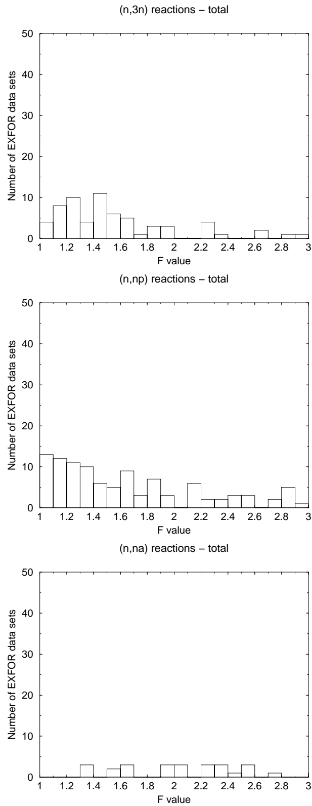
Figure 7: Distribution of F-values for the (n,3n), (n,np) and (n,na) reactions.
