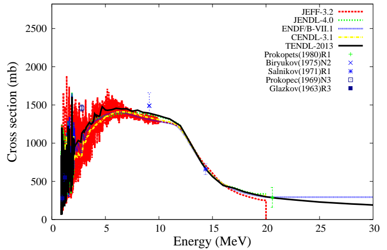
^{59}\text{Co}(n,n)^{59}\text{Co}
