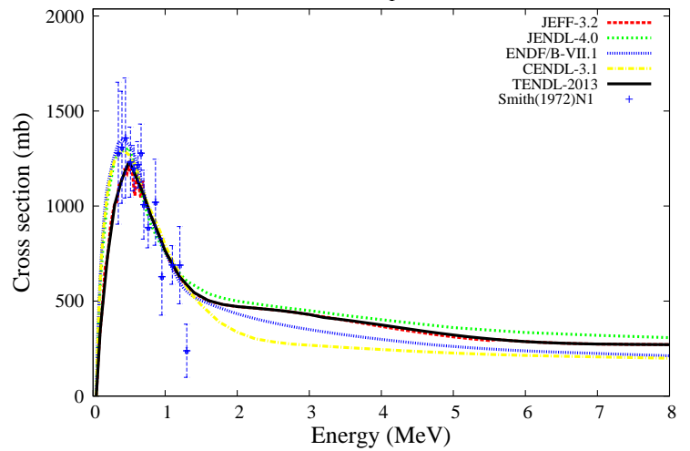
^{240}\text{Pu}(n,n_1)^{240}\text{Pu}
