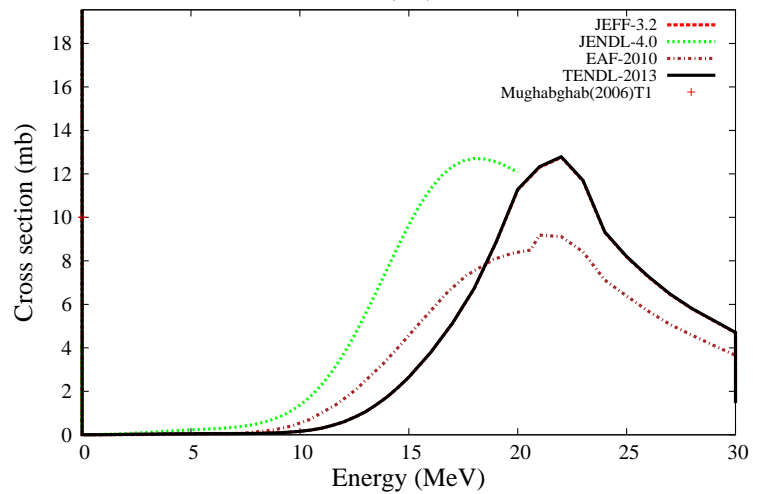
^{188}\text{Os}(n,a)^{185}\text{W}
