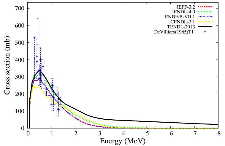
^{200}\text{Hg}(n,n_1)^{200}\text{Hg}
