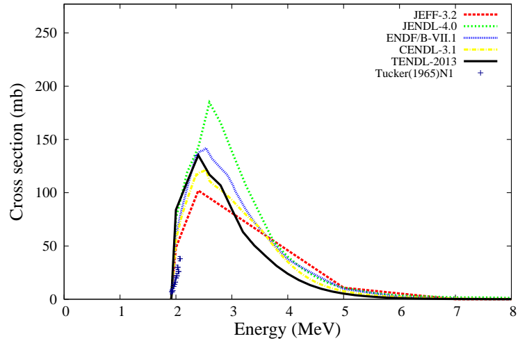
^{150}\text{Nd}(n,n_2')^{150}\text{Nd}
