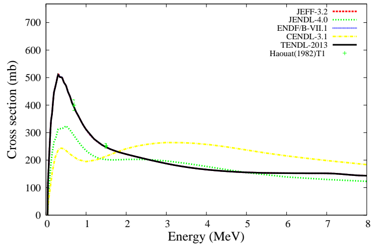
^{238}\text{U}(n,n_1)^{238}\text{U}
