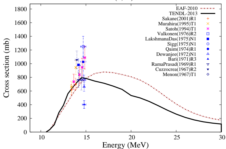
^{144}\text{Sm}(n,2n)^{143g}\text{Sm}
