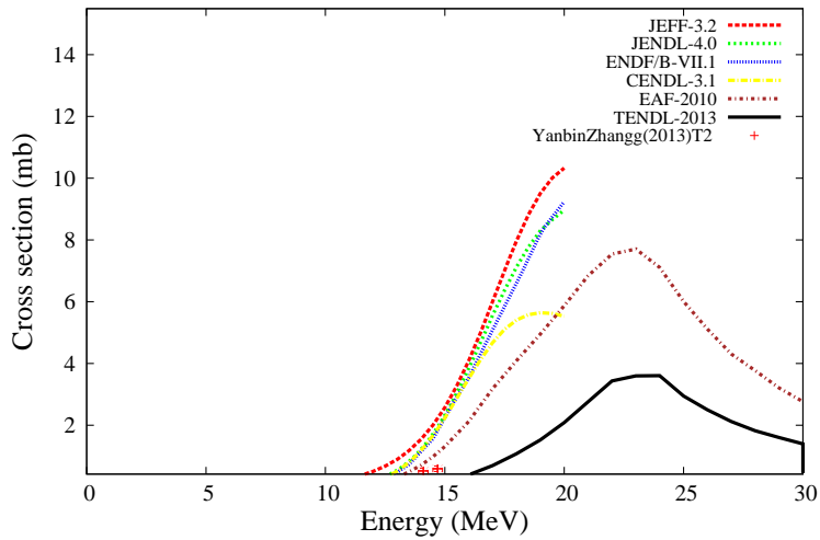
^{156}\text{Dy}(n,a)^{153}\text{Gd}
