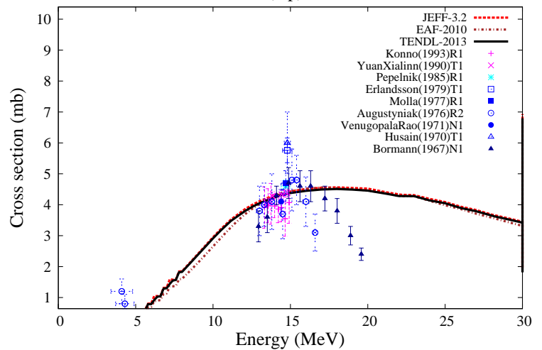
^{85}\text{Rb}(n,p)^{85m}\text{Kr}
