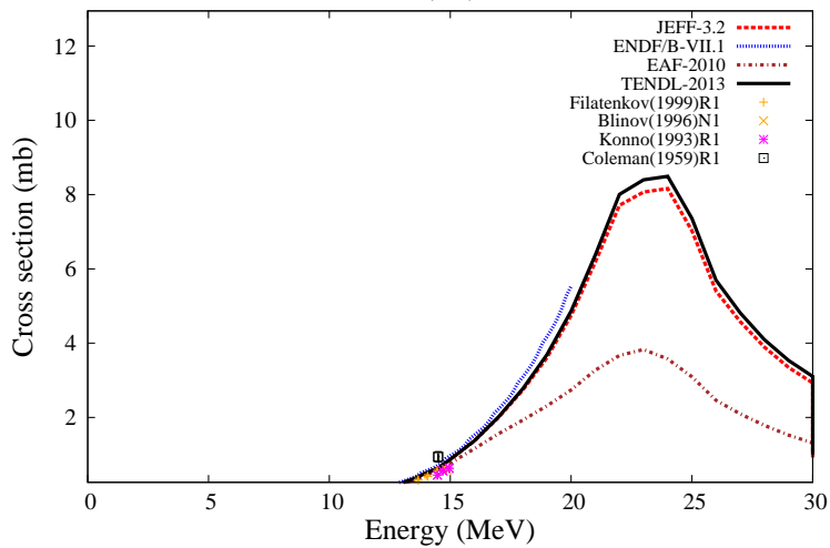
^{187}\text{Os}(n,a)^{184}\text{W}
