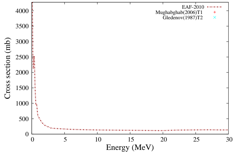
{}^{11}\text{B}(n,p){}^{11}\text{Be}
