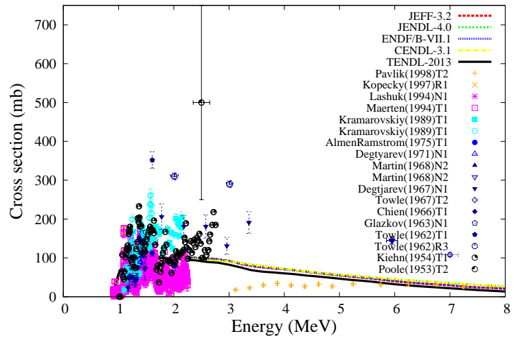
^{31}\text{P}(n,n_1')^{31}\text{P}
