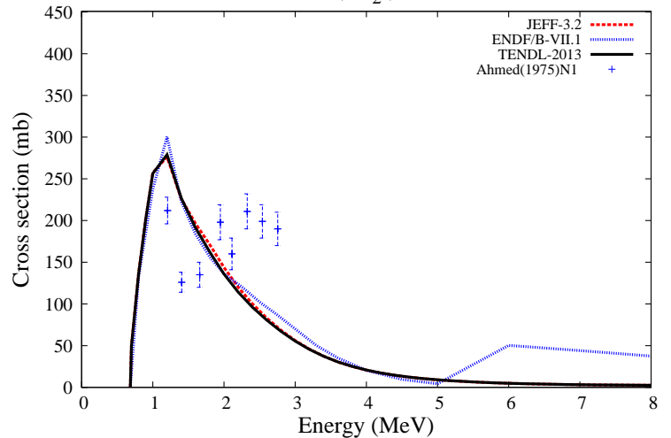
^{207}\text{Pb}(n,n_2')^{207}\text{Pb}
