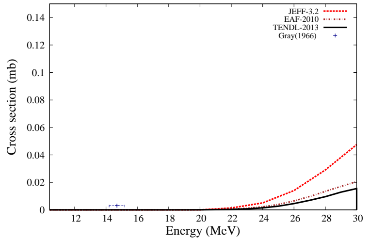
^{127}\text{I}(n,2p)^{126}\text{Sb}
