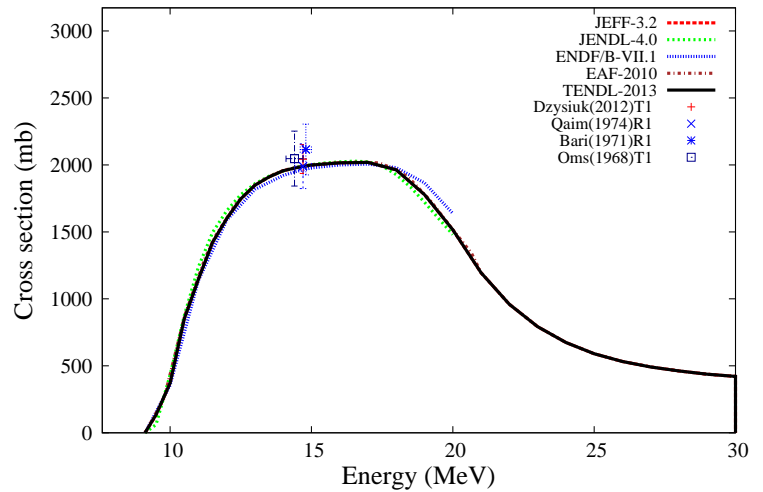
^{165}\text{Ho}(n,2n)^{164}\text{Ho}
