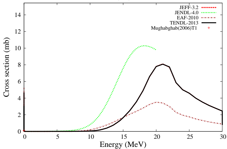
^{187}\text{Os}(n,a)^{184}\text{W}
