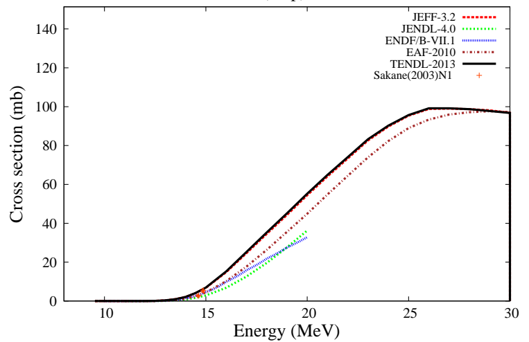
^{88}\text{Zr}(n,np)^{87}\text{Y}
