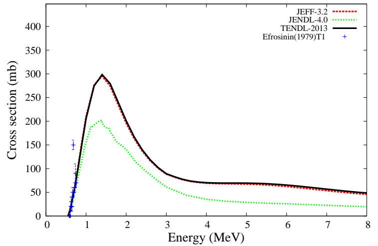
^{203}\text{Tl}(n,n_2')^{203}\text{Tl}
