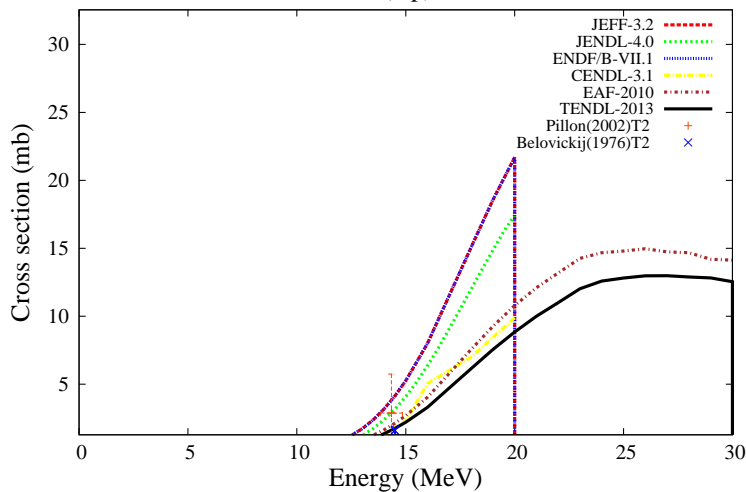
^{209}\text{Bi}(n,p)^{209}\text{Pb}
