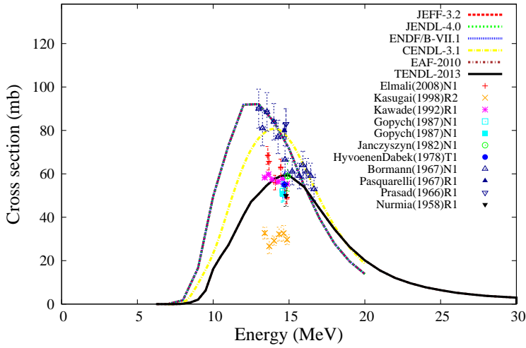
^{27}\text{Al}(n,a)^{24}\text{Na}
