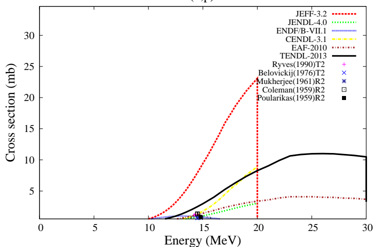
^{209}\text{Bi}(n,p)^{209}\text{Pb}
