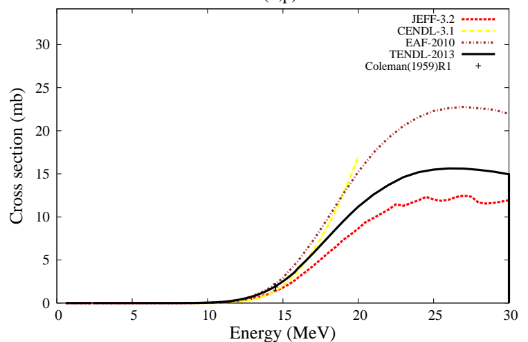
^{235}\text{U}(n,p)^{235}\text{Pa}
