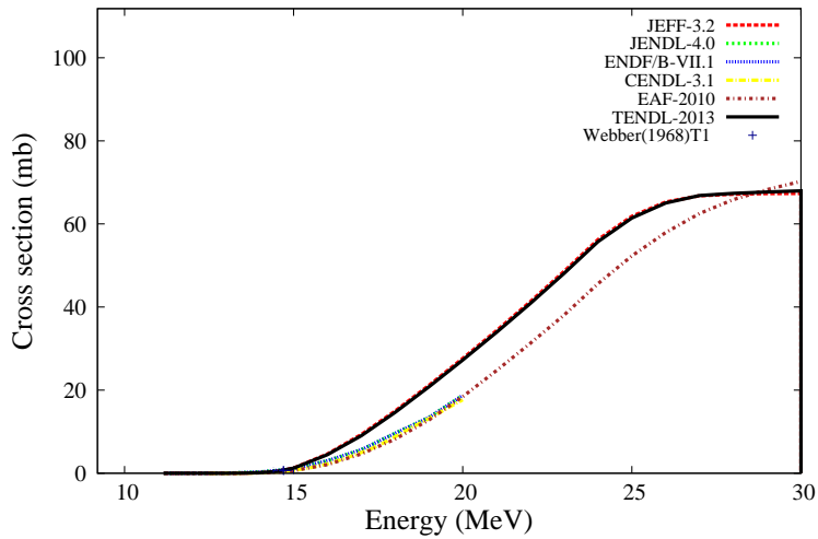
^{84}\text{Sr}(n,np)^{83}\text{Rb}
