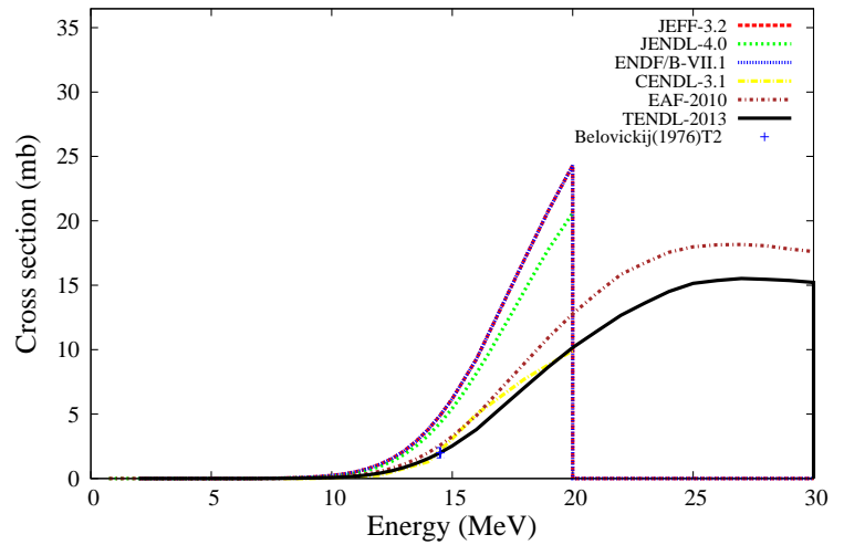
^{208}\text{Pb}(n,p)^{208}\text{Tl}
