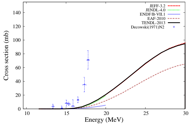
^{87}\text{Sr}(n,np)^{86}\text{Rb}
