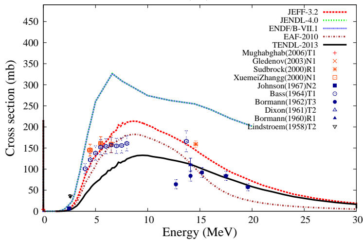
^{41}\text{K}(n,a)^{38}\text{Cl}
