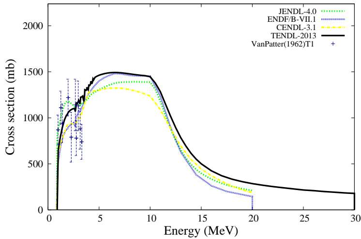
^{56}\text{Fe}(n,n)^{56}\text{Fe}
