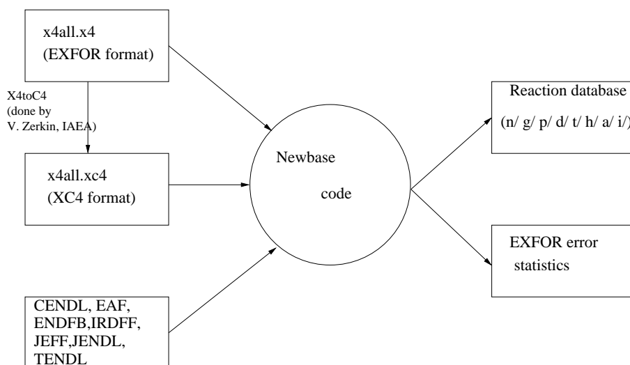
Figure 1: Databases produced out of EXFOR.
