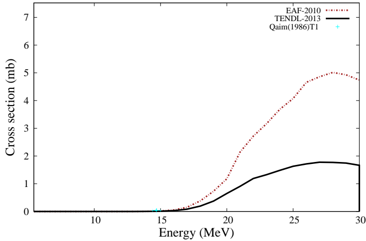
^{159}\text{Tb}(n,n\alpha)^{155}\text{Eu}
