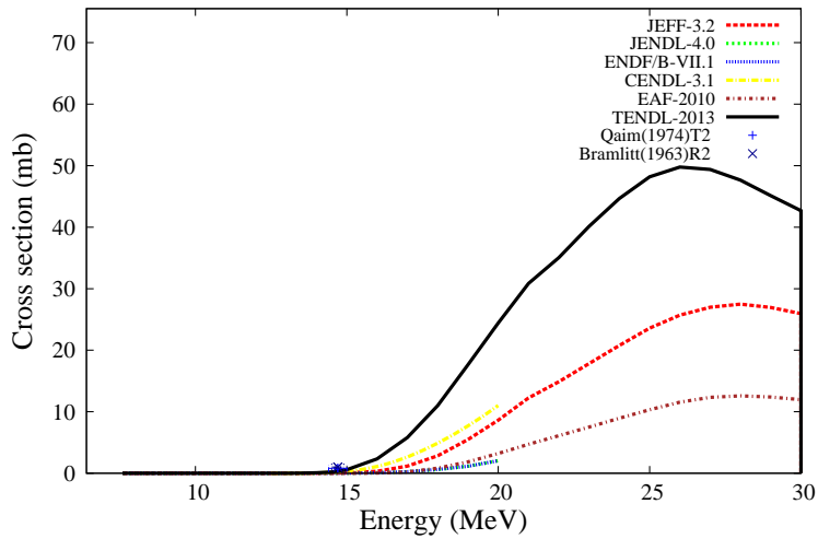
^{87}\text{Rb}(n,\text{na})^{83}\text{Br}
