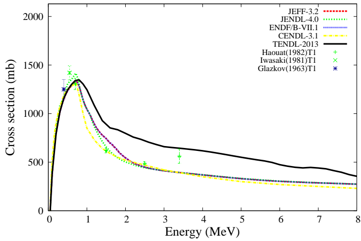
^{235}\text{U}(n,n_1)^{235}\text{U}
