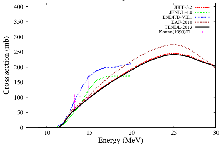
^{87}\text{Sr}(n,np)^{86m}\text{Rb}
