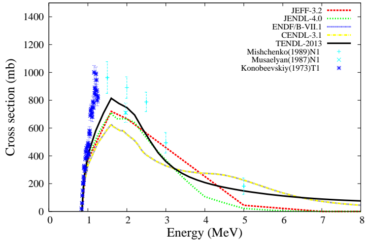
^{134}\text{Ba}(n,n_1)^{134}\text{Ba}
