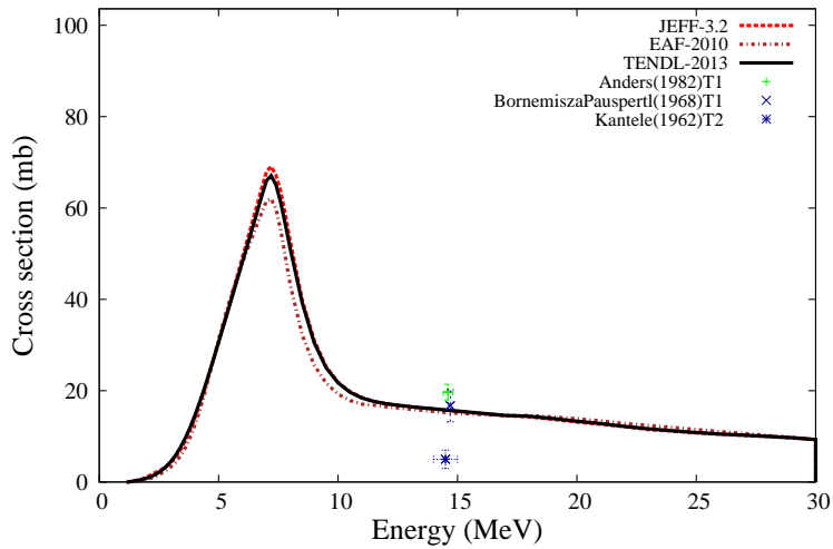
^{180}\text{Hf}(n,n)^{180\text{m}}\text{Hf}
