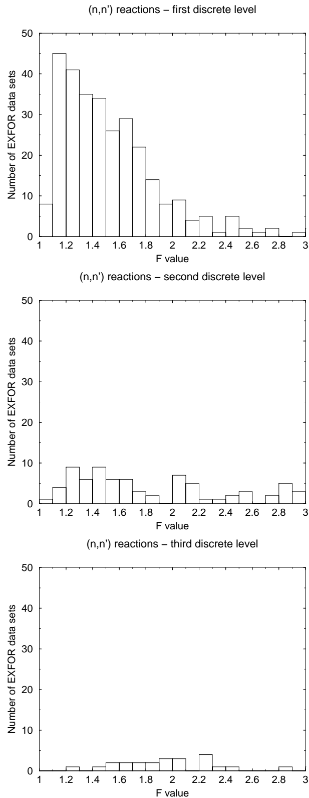
Figure 6: Distribution of F-values for the (n,n') reaction to discrete levels.
