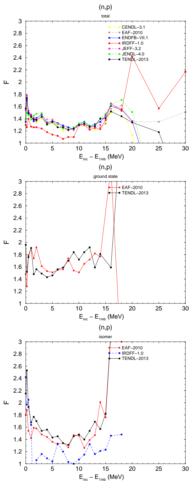
Figure 10: F values, averaged over all nuclides, for (n,p) reactions as a function of incident energy, for the various nuclear data libraries. E_{1mb} is an estimate for the threshold energy and is the incident energy where the cross section crosses the 1 mb value.
