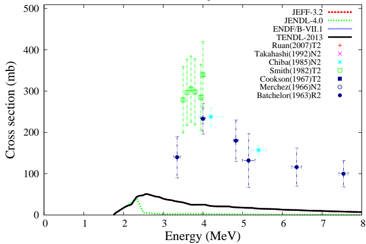
{}^9\text{Be}(n,n_1){}^9\text{Be}
