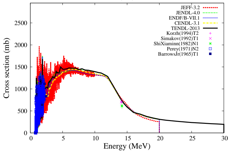
^{60}\text{Co}(n,n)^{60}\text{Co}
