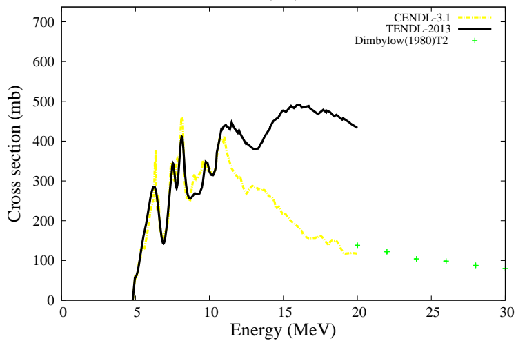
{}^{12}\text{C}(n,n){}^{12}\text{C}
