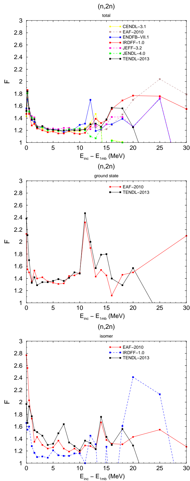
Figure 9: F values, averaged over all nuclides, for (n,2n) reactions as a function of incident energy, for the various nuclear data libraries. E_{1mb} is an estimate for the threshold energy and is the incident energy where the cross section crosses the 1 mb value.
