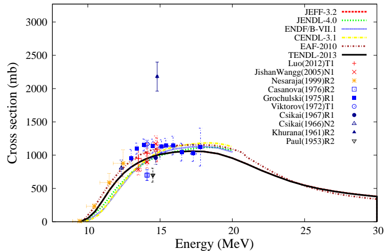
^{72}\text{Ge}(n,2n)^{71}\text{Ge}
