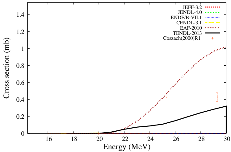
^{41}\text{K}(n,2p)^{40}\text{Cl}
