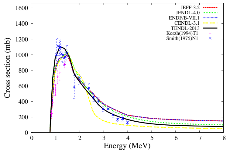
^{100}\text{Mo}(n,n_1)^{100}\text{Mo}
