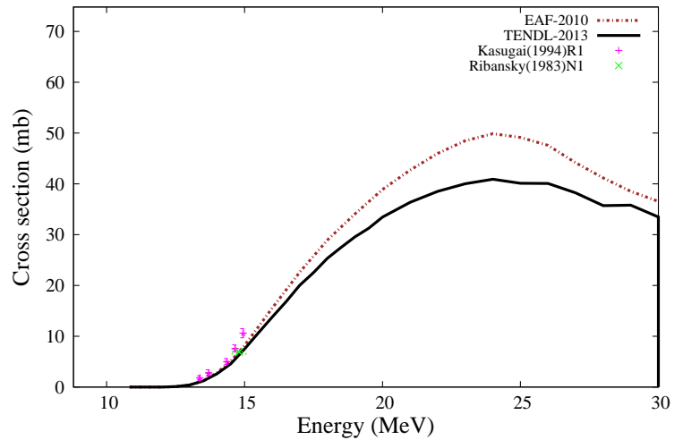
^{49}\text{Ti}(n,np)^{48}\text{Sc}
