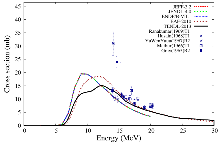
^{40}\text{K}(n,a)^{37}\text{Cl}
