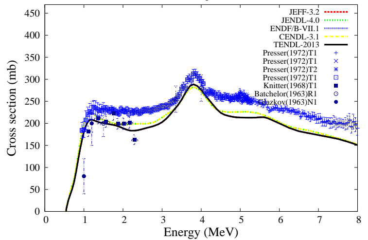
{}^{10}\text{B}(n,n_1){}^{10}\text{B}
