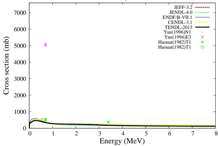
^{239}\text{Pu}(n,n_1)^{239}\text{Pu}
