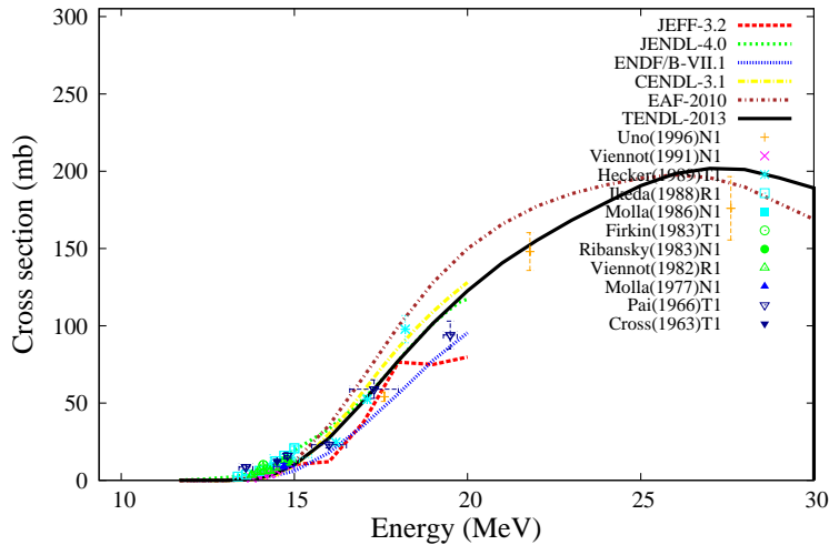
^{48}\text{Ti}(n,np)^{47}\text{Sc}
