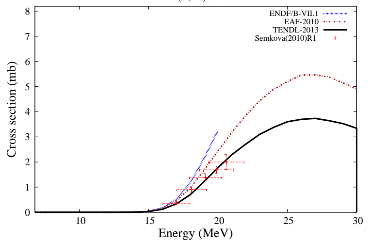
^{93}\text{Nb}(n,\text{na})^{89\text{m}}\text{Y}
