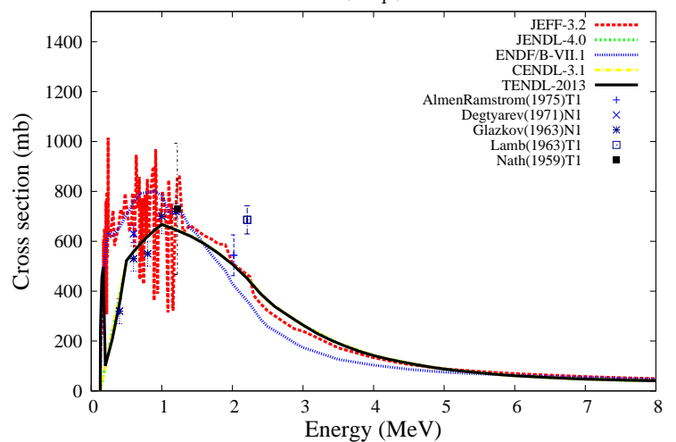
^{56}\text{Fe}(n,n_1)^{56}\text{Fe}
