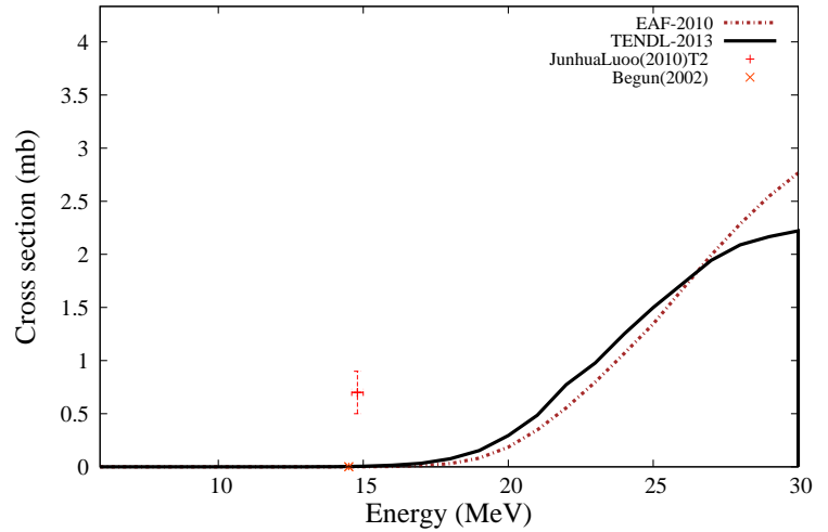
^{165}\text{Ho}(n,n\alpha)^{161}\text{Tb}
