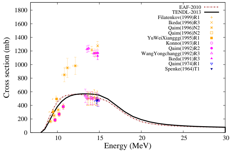
^{153}\text{Eu}(n,2n)^{152\text{g}}\text{Eu}
