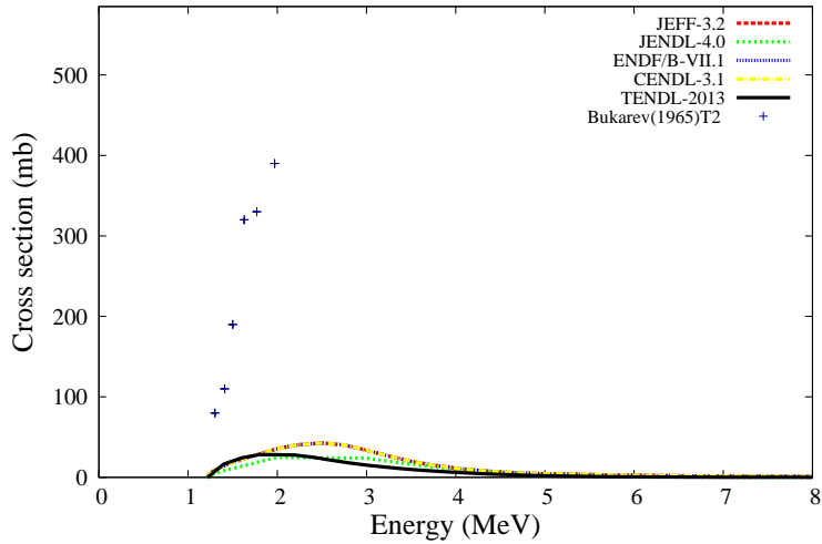
^{141}\text{Pr}(n,n_2')^{141}\text{Pr}
