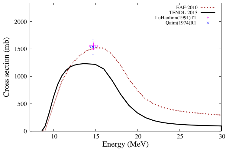
^{152}\text{Gd}(n,2n)^{151}\text{Gd}
