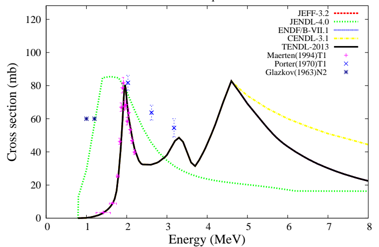
{}^{10}\text{B}(n,n_1){}^{10}\text{B}
