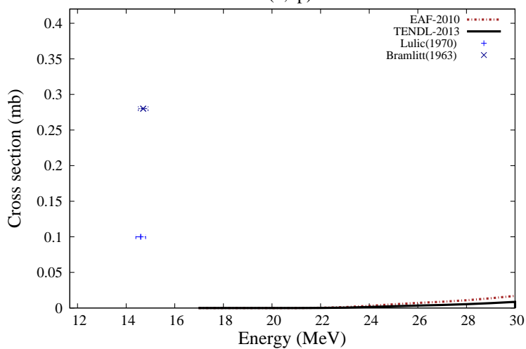
^{50}\text{Ti}(n,2p)^{49}\text{Ca}
