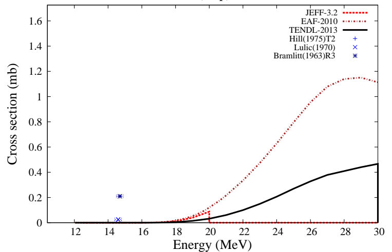
^{51}\text{V}(n,2p)^{50}\text{Sc}
