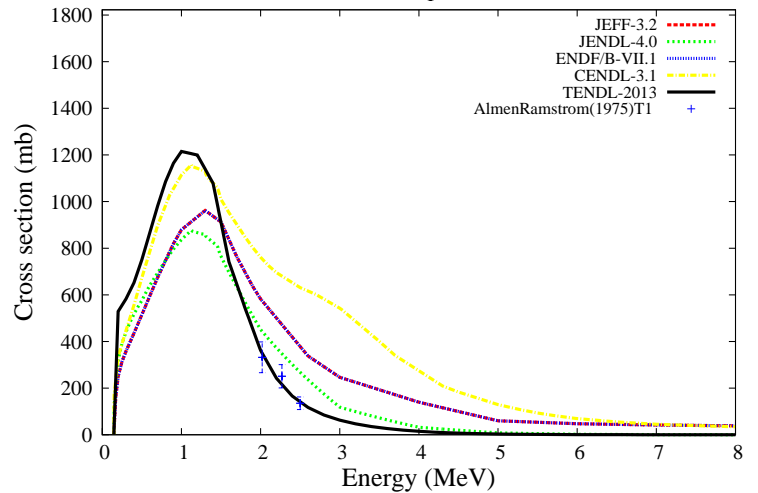
^{141}\text{Pr}(n,n_1)^{141}\text{Pr}
