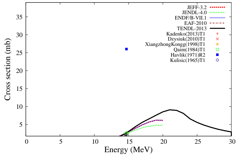
^{161}\text{Dy}(n,a)^{158}\text{Gd}
