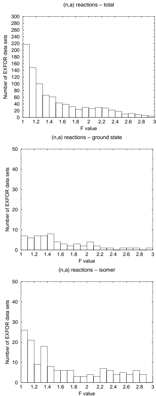
Figure 4: Distribution of F-values for the (n, \alpha ) reaction.
