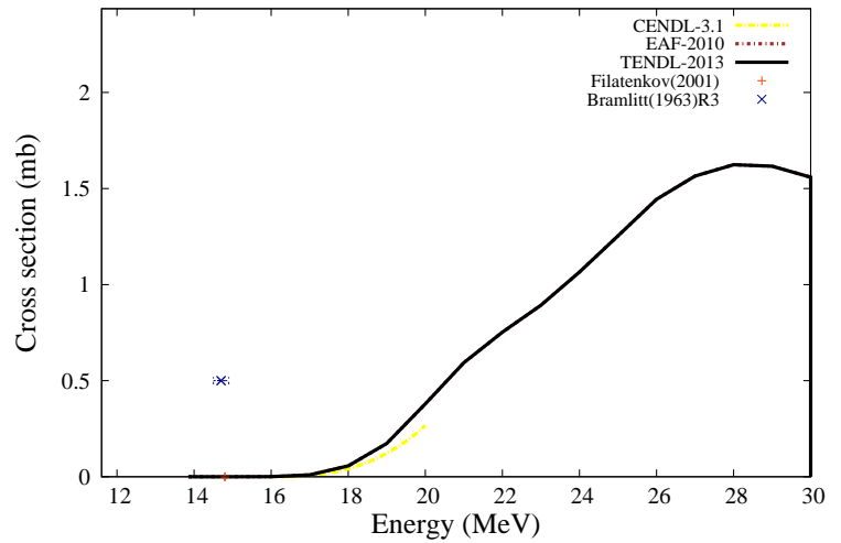
^{45}\text{Sc}(n,2p)^{44}\text{K}
