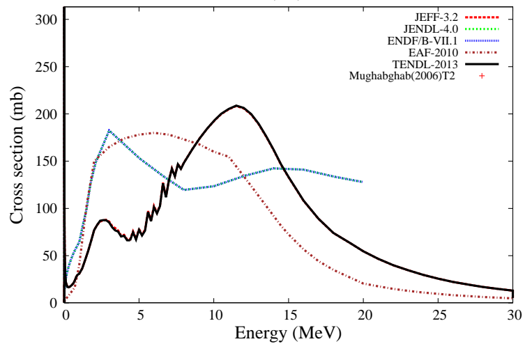
^{40}\text{Ca}(n,a)^{37}\text{Ar}
