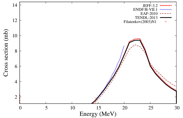
^{184}\text{Os}(n,a)^{181}\text{W}
