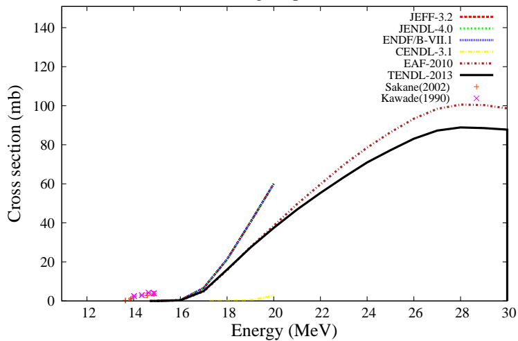
^{26}\text{Mg}(n,np)^{25}\text{Na}
