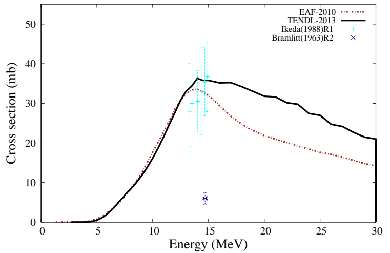
^{95}\text{Mo}(n,p)^{95g}\text{Nb}
