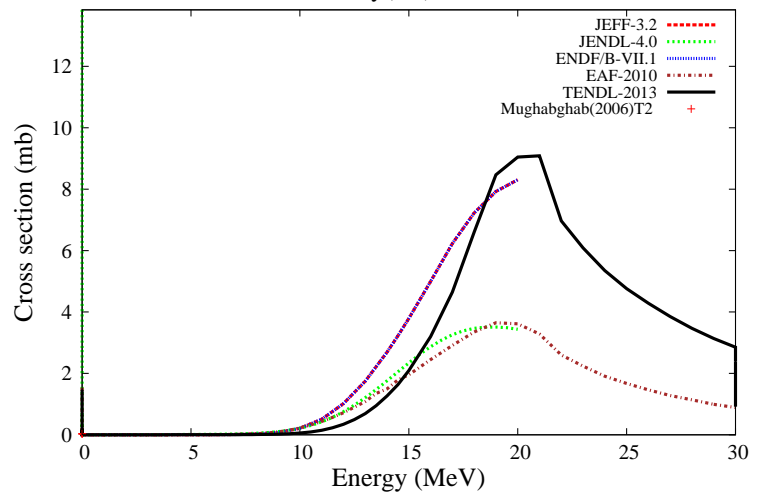
^{163}\text{Dy}(n,a)^{160}\text{Gd}
