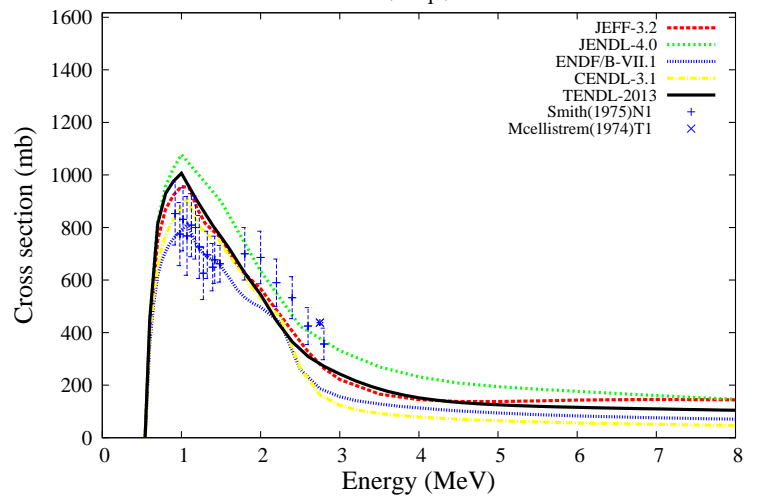
^{100}\text{Mo}(n,n_1)^{100}\text{Mo}
