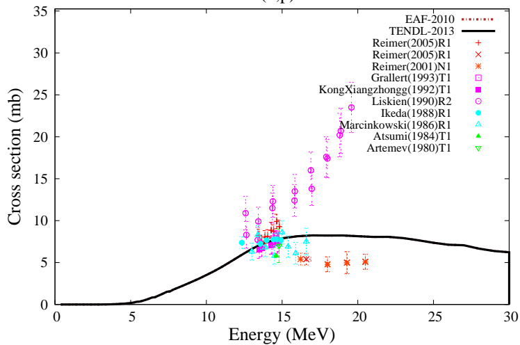
^{95}\text{Mo}(n,p)^{95m}\text{Nb}
