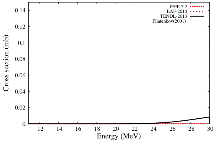
^{103}\text{Rh}(n,2p)^{102\text{m}}\text{Tc}
