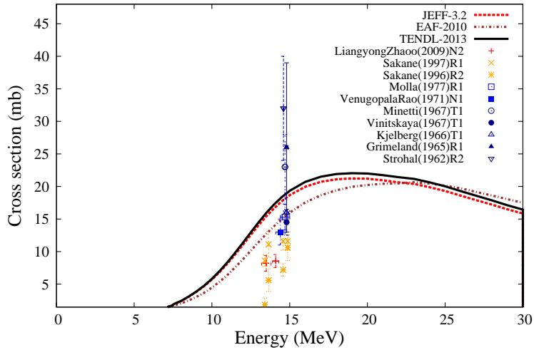
^{82}\text{Kr}(n,p)^{82}\text{Br}
