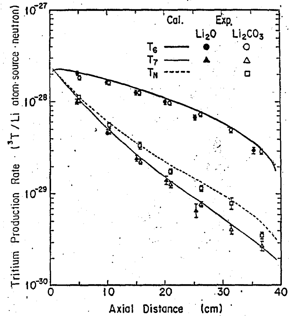
Fig. 5 Tritium production-rate distribution in 40 cm thick \text{Li}_2\text{O} slab assembly.
