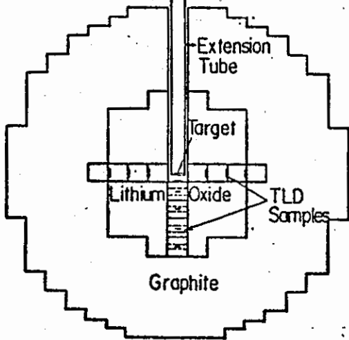
Fig. 1 Horizontal section across the center of \text{Li}_2\text{O-C} assembly
