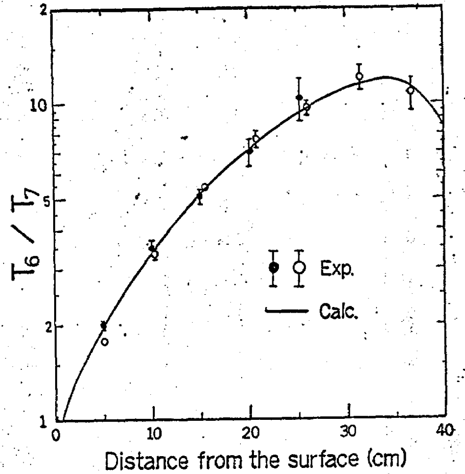
Fig. 6 T_6 / T_7 ratio distribution in 40 cm thick \text{Li}_2\text{O} slab assembly
