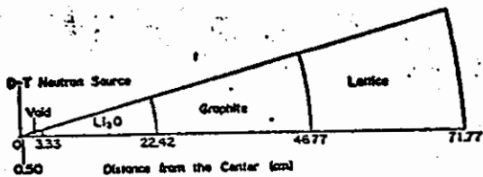
Fig. 2 Calculational model of \text{Li}_2\text{O-C} assembly
