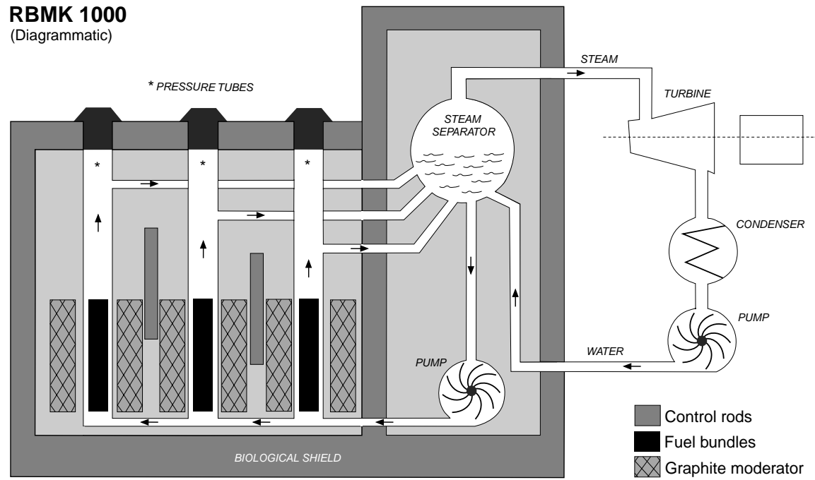
Figure 2. The RBMK reactor
